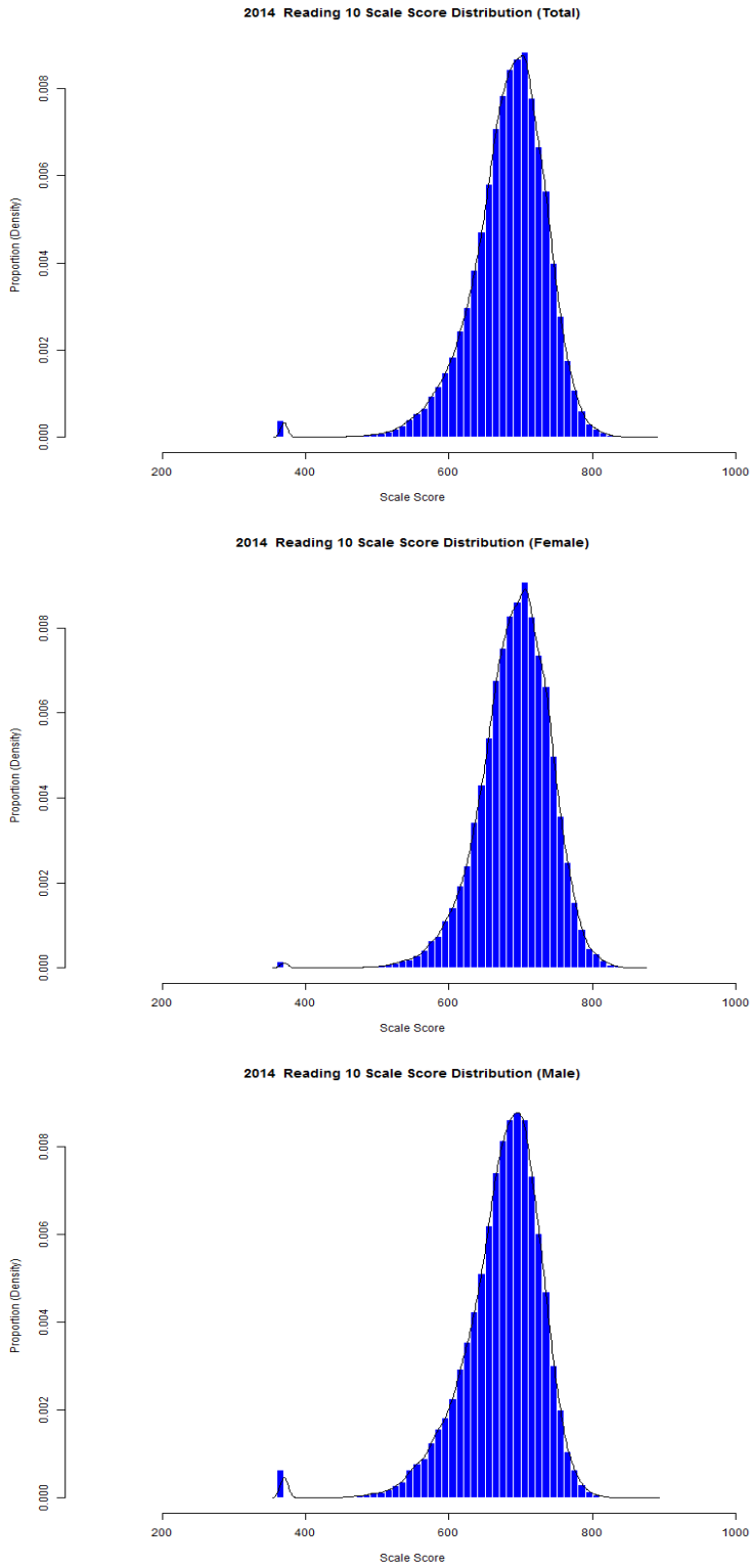
Figure 50. Grade 10 Reading Scale Score Distributions for the Total Population, Female, and Male Students
