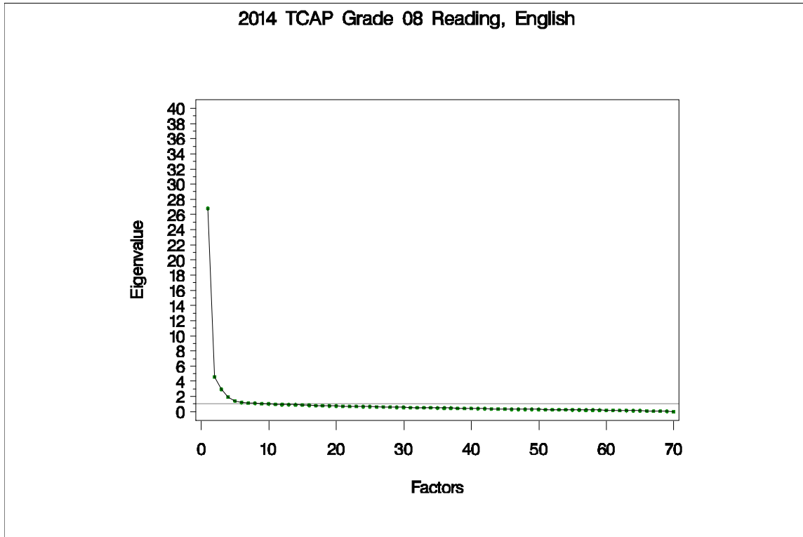
Figure 60. Eigenvalues and Proportions of Variance by Factor for TCAP Grade 8 Reading
