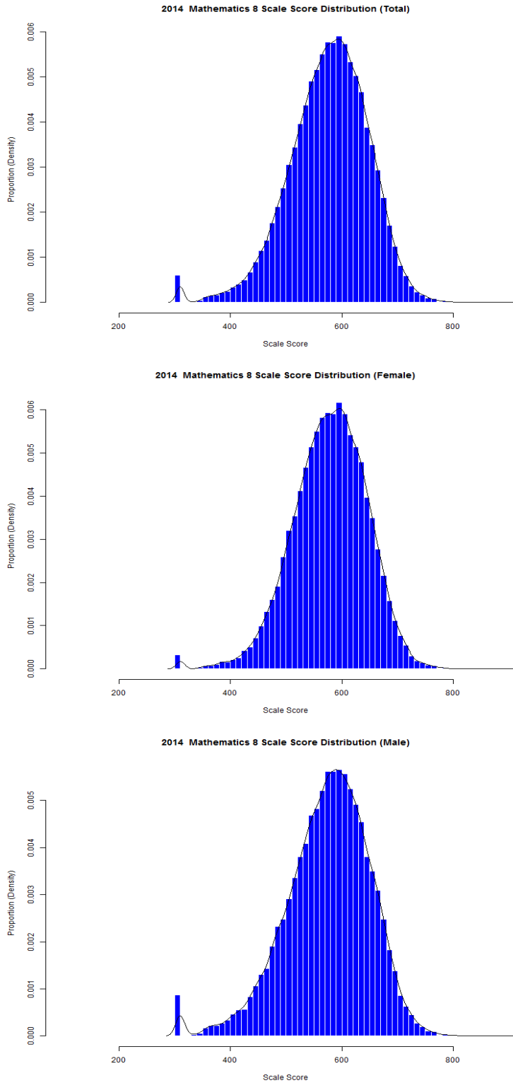
Figure 46. Grade 8 Mathematics Scale Score Distributions for the Total Population, Female, and Male Students
