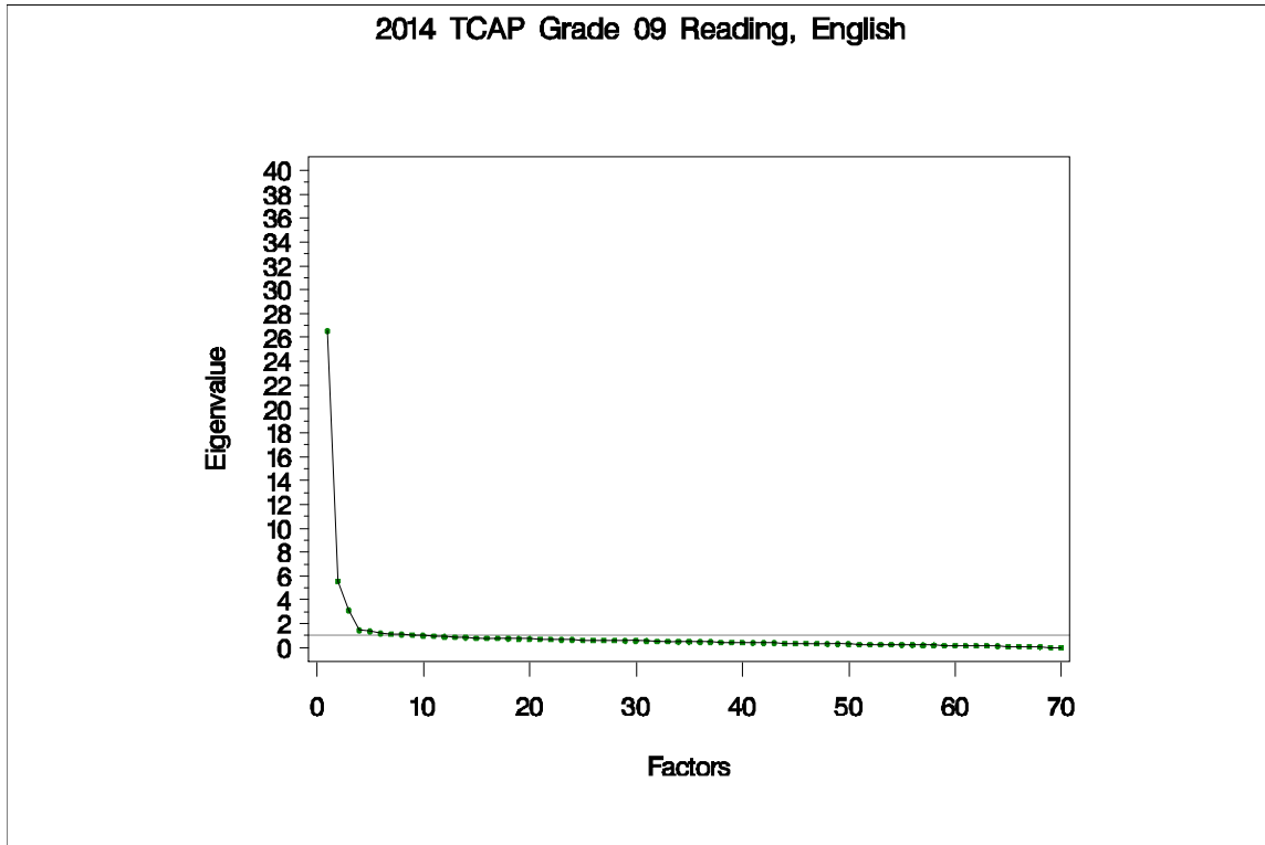
Figure 61. Eigenvalues and Proportions of Variance by Factor for TCAP Grade 9 Reading
