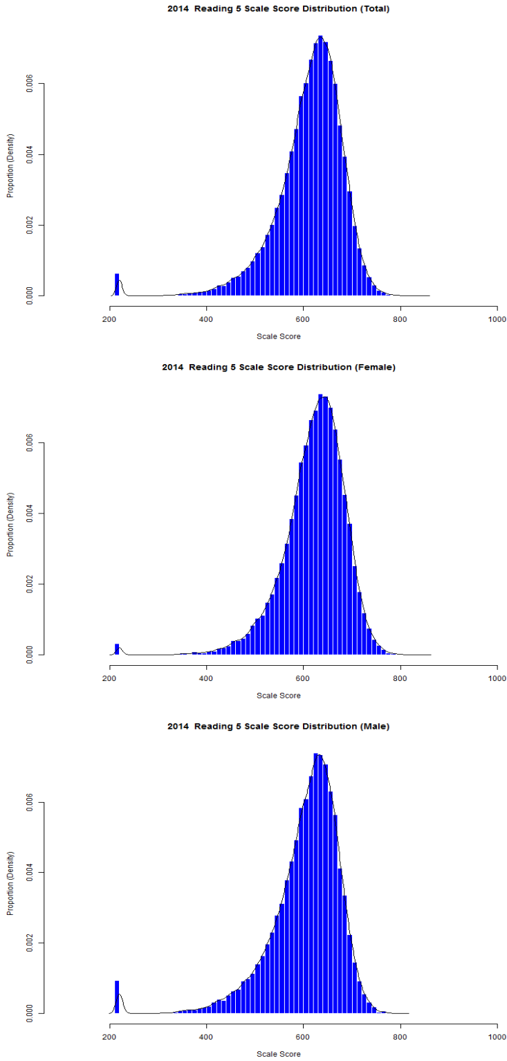
Figure 35. Grade 5 Reading Scale Score Distributions for the Total Population, Female, and Male Students
