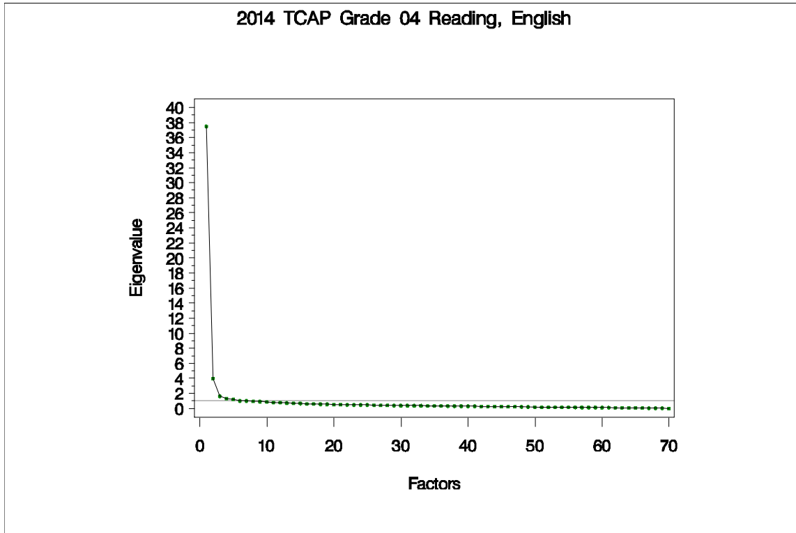
Figure 55. Eigenvalues and Proportions of Variance by Factor for TCAP Grade 4 Reading
