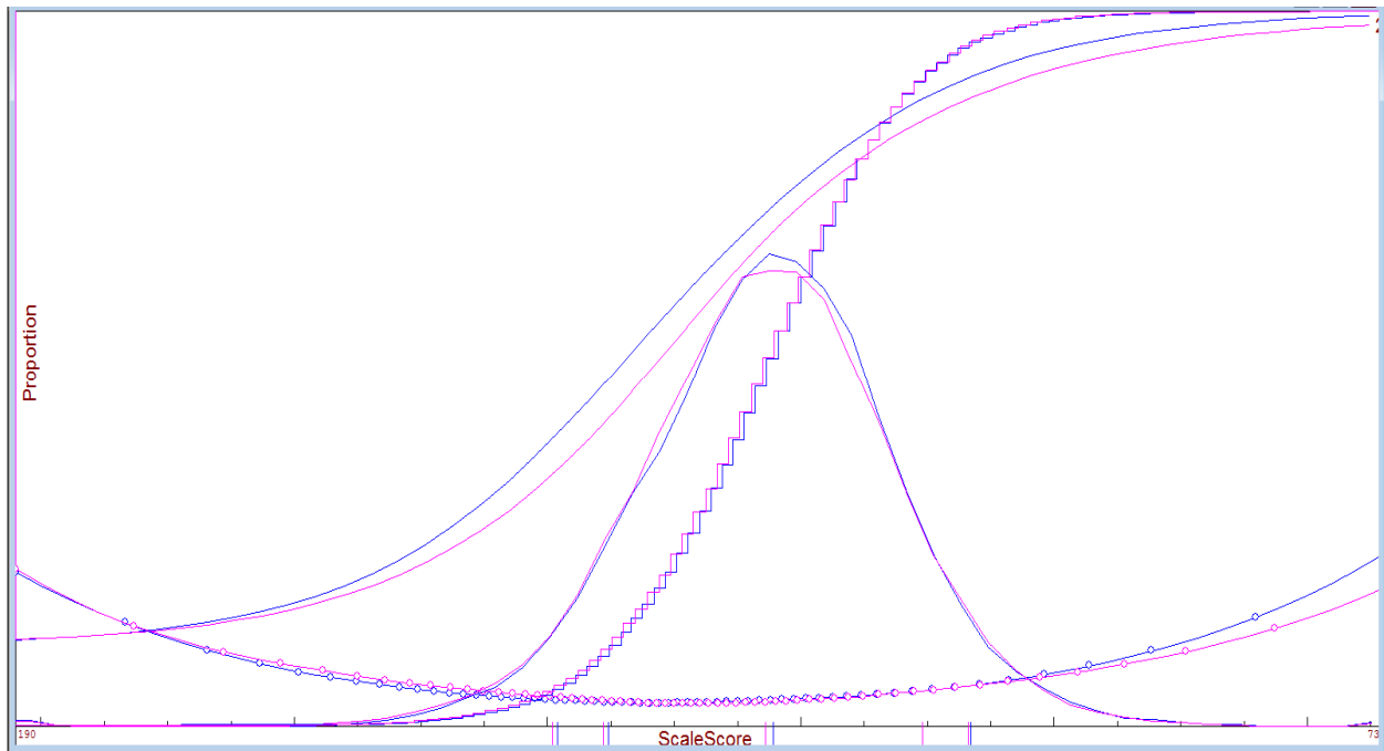
Figure 10. TCAP Grade 4 Writing Operational Tests
