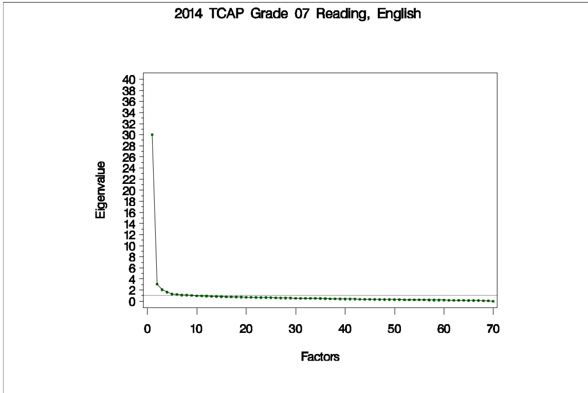
Figure 59. Eigenvalues and Proportions of Variance by Factor for TCAP Grade 7 Reading
