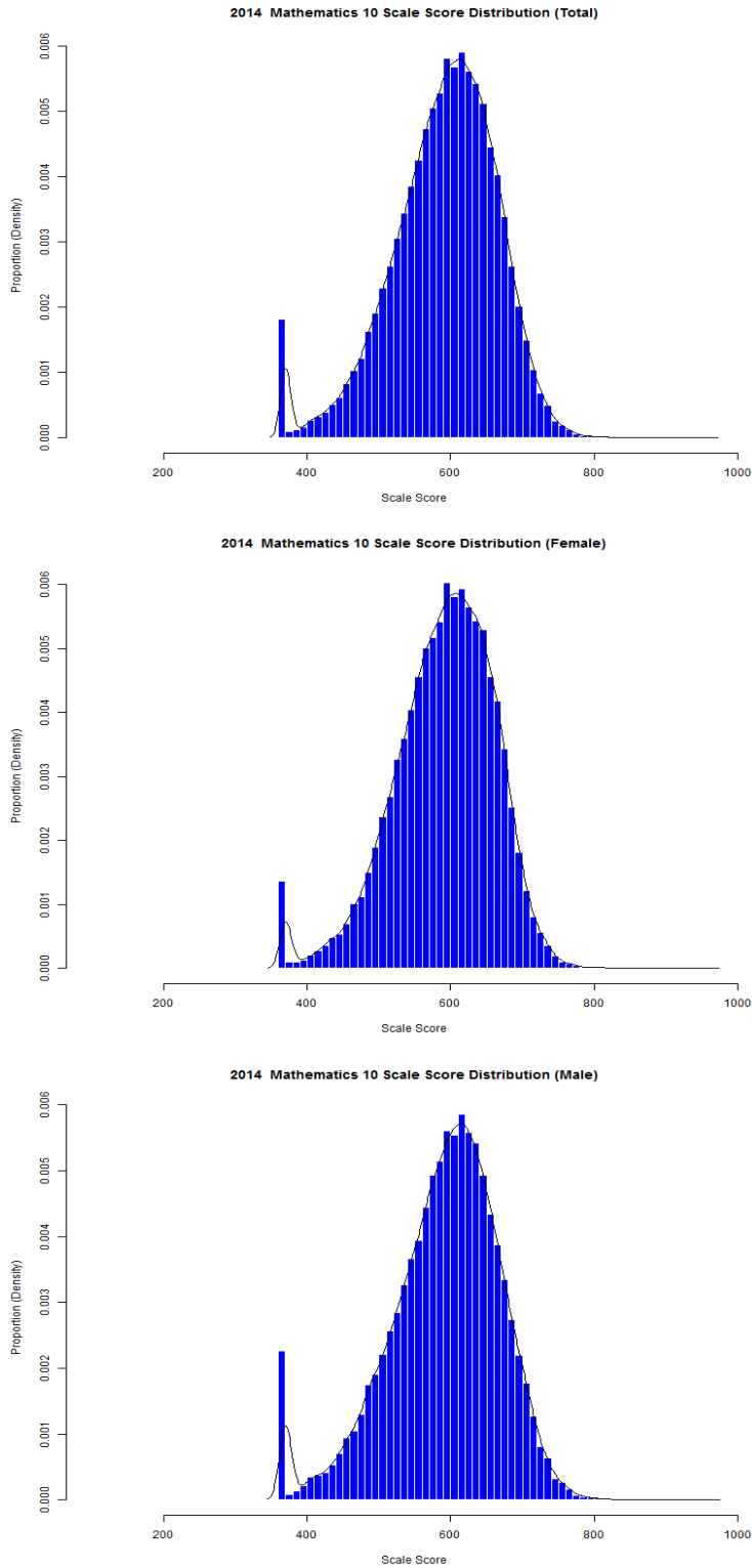
Figure 52. Grade 10 Mathematics Scale Score Distributions for the Total Population, Female, and Male Students
