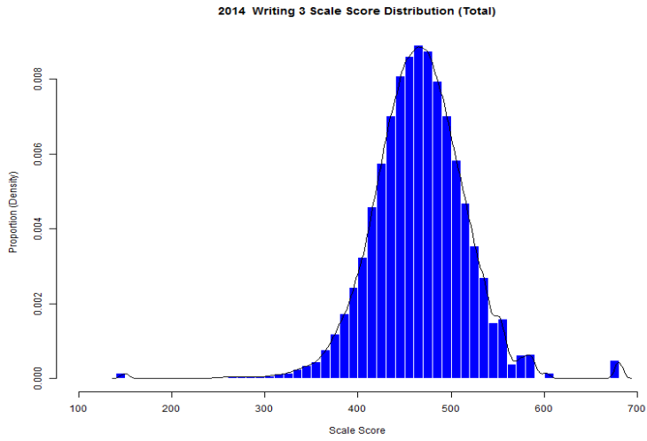
Figure 27. Grade 3 Writing Scale Score Distributions for the Total Population, Female, and Male Students
