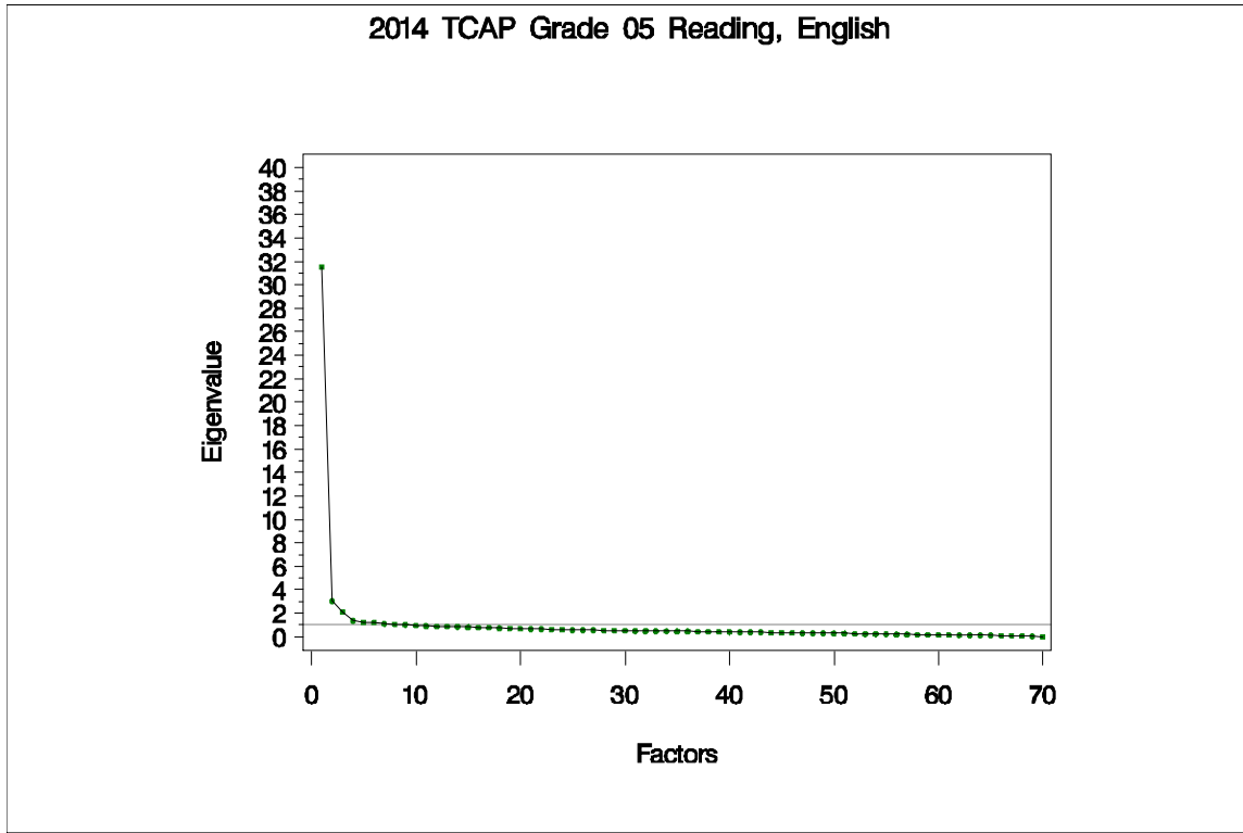
Figure 57. Eigenvalues and Proportions of Variance by Factor for TCAP Grade 5 Reading
