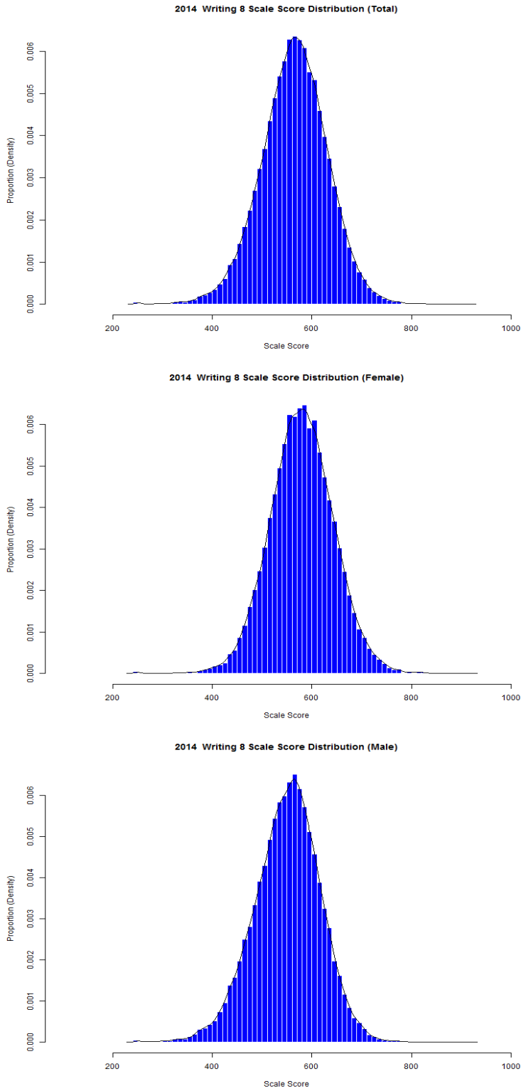
Figure 45. Grade 8 Writing Scale Score Distributions for the Total Population, Female, and Male Students
