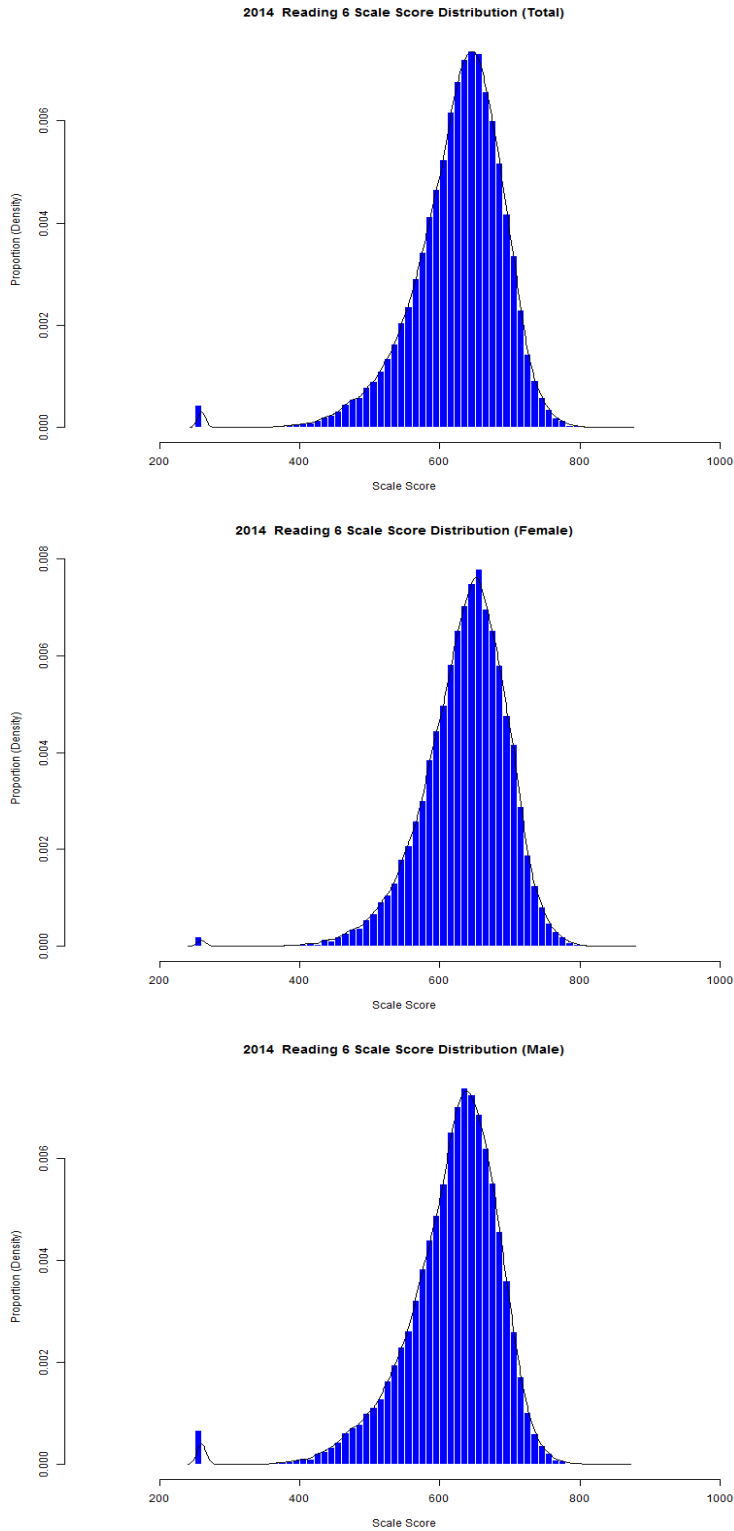
Figure 38. Grade 6 Reading Scale Score Distributions for the Total Population, Female, and Male Students
