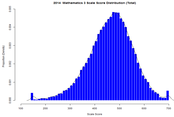
Figure 29. Grade 3 Mathematics Scale Score Distributions for the Total Population, Female, and Male Students
