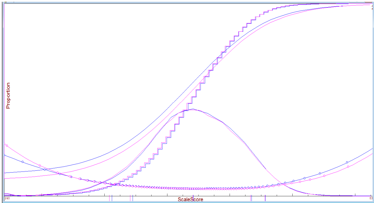
Figure 20. TCAP Grade 6 Mathematics Operational Tests
