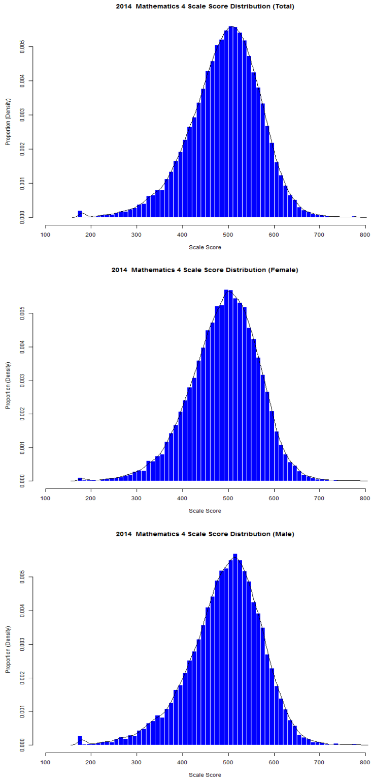
Figure 34. Grade 4 Mathematics Scale Score Distributions for the Total Population, Female, and Male Students
