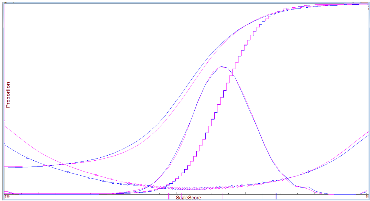
Figure 9. TCAP Grade 3 Writing Operational Tests
