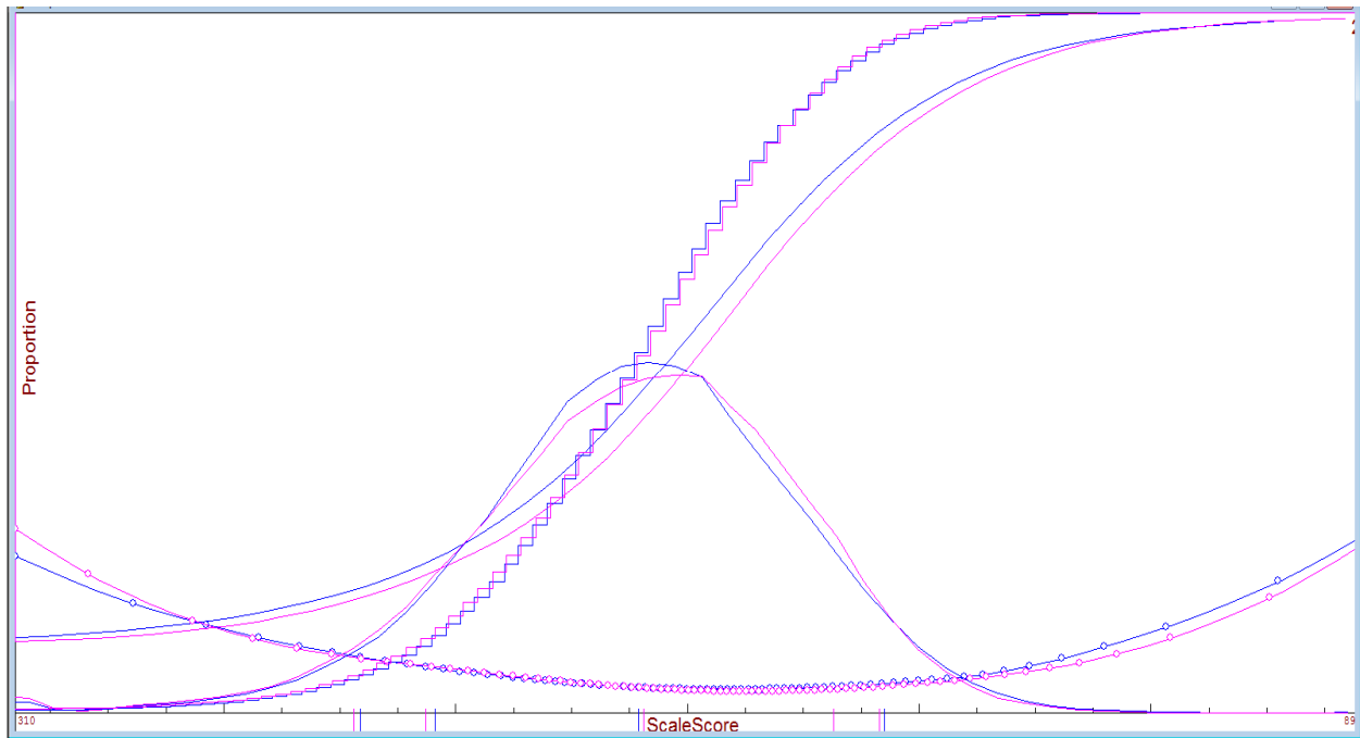
Figure 22. TCAP Grade 8 Mathematics Operational Tests
