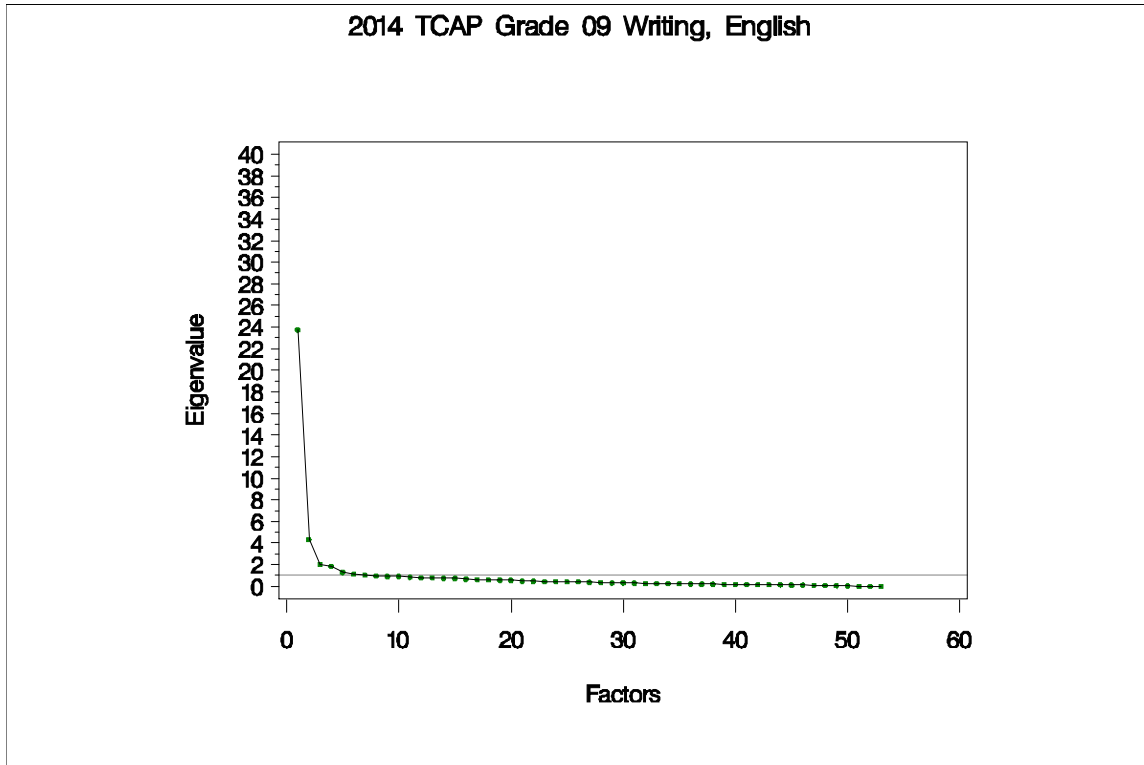
Figure 71. Eigenvalues and Proportions of Variance by Factor for TCAP Grade 9 Writing
