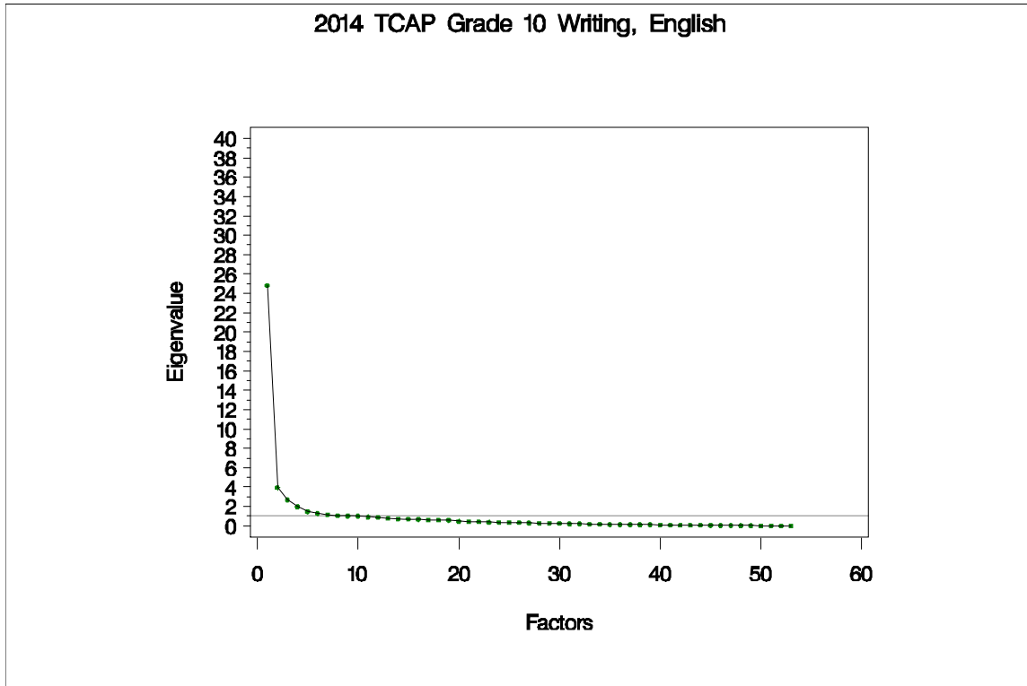
Figure 72. Eigenvalues and Proportions of Variance by Factor for TCAP Grade 10 Writing
