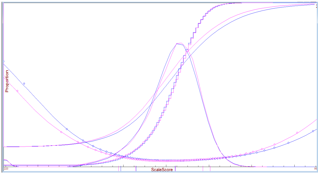
Figure 3. TCAP Grade 5 Reading Operational Tests
