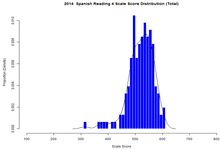
Figure 31. Grade 4 Reading (Spanish) Scale Score Distributions for the Total Population, Female, and Male Students
