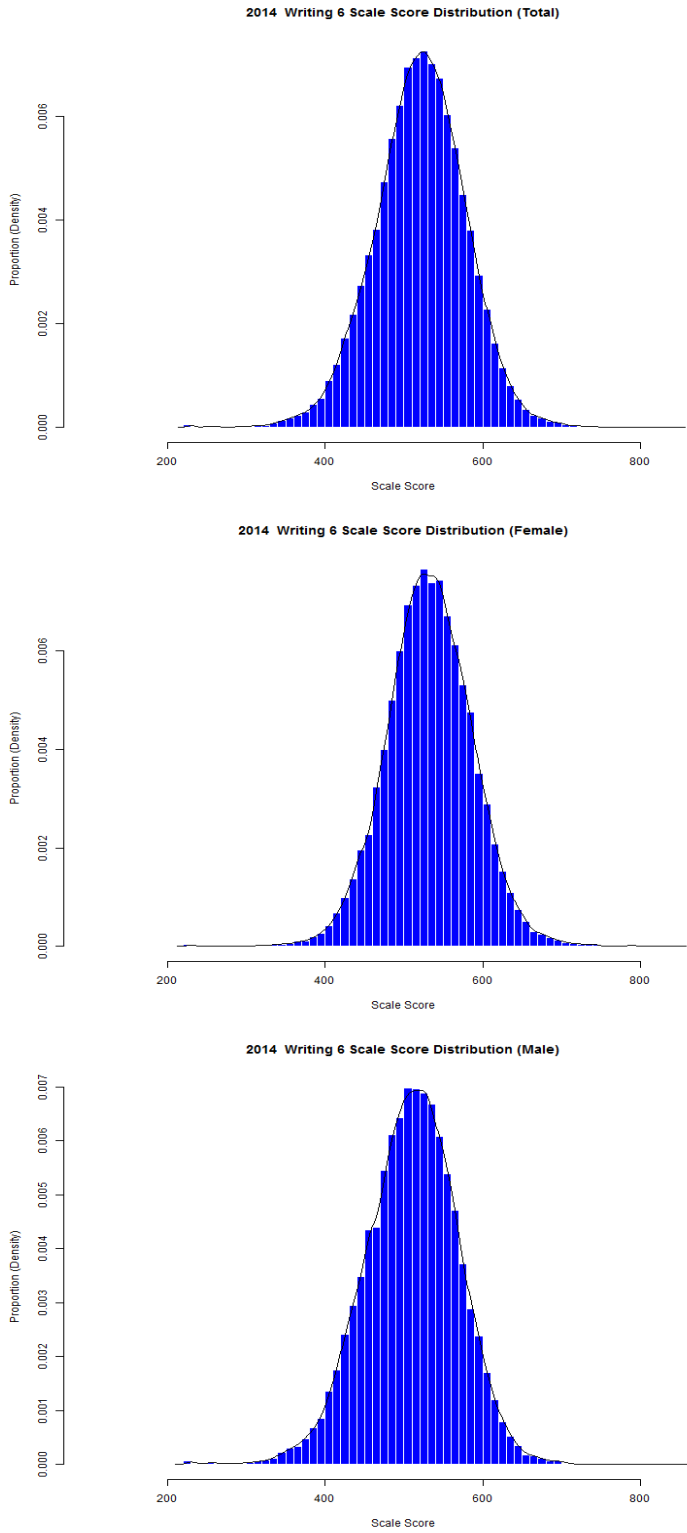
Figure 39. Grade 6 Writing Scale Score Distributions for the Total Population, Female, and Male Students
