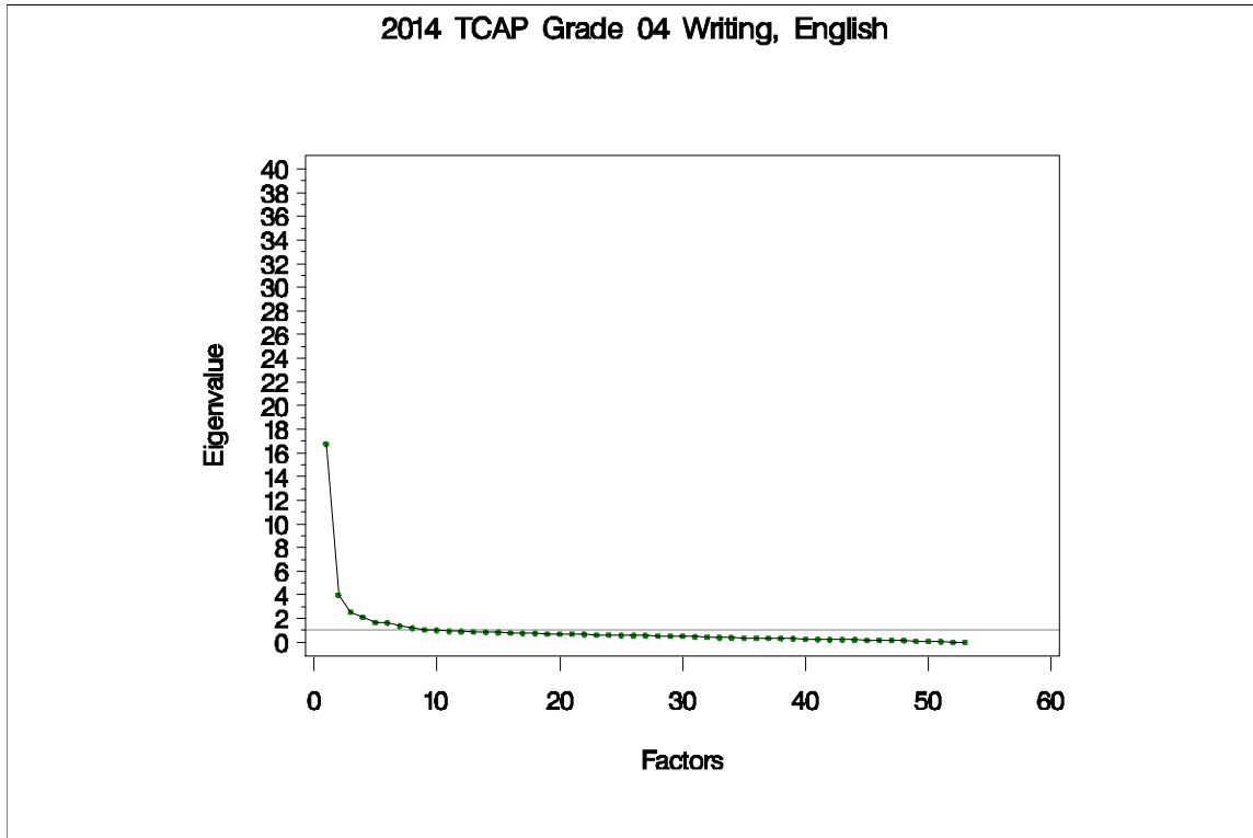
Figure 65. Eigenvalues and Proportions of Variance by Factor for TCAP Grade 4 Writing
