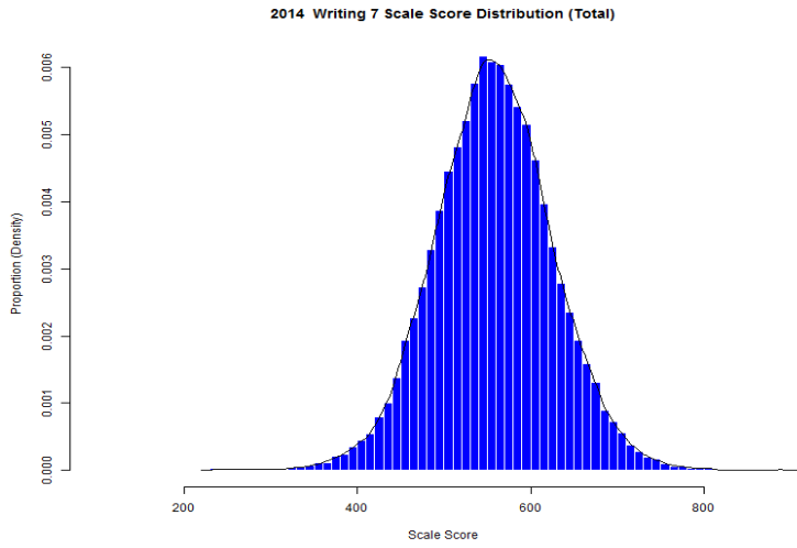
Figure 42. Grade 7 Writing Scale Score Distributions for the Total Population, Female, and Male Students
