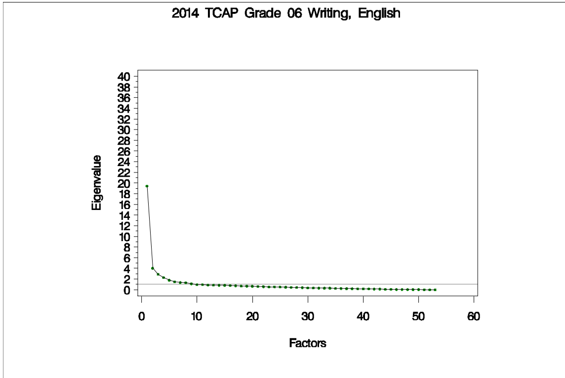
Figure 68. Eigenvalues and Proportions of Variance by Factor for TCAP Grade 6 Writing
