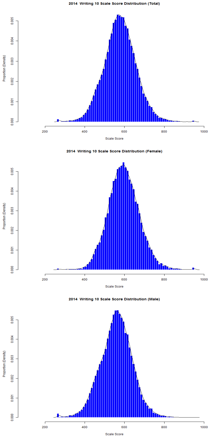
Figure 51. Grade 10 Writing Scale Score Distributions for the Total Population, Female, and Male Students
