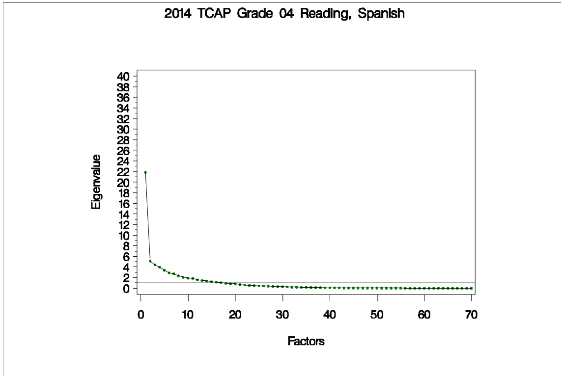
Figure 56. Eigenvalues and Proportions of Variance by Factor for TCAP Grade 4 Reading (Spanish)
