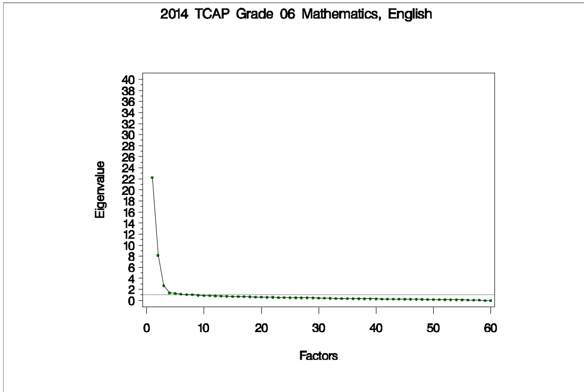
Figure 76. Eigenvalues and Proportions of Variance by Factor for TCAP Grade 6 Mathematics
