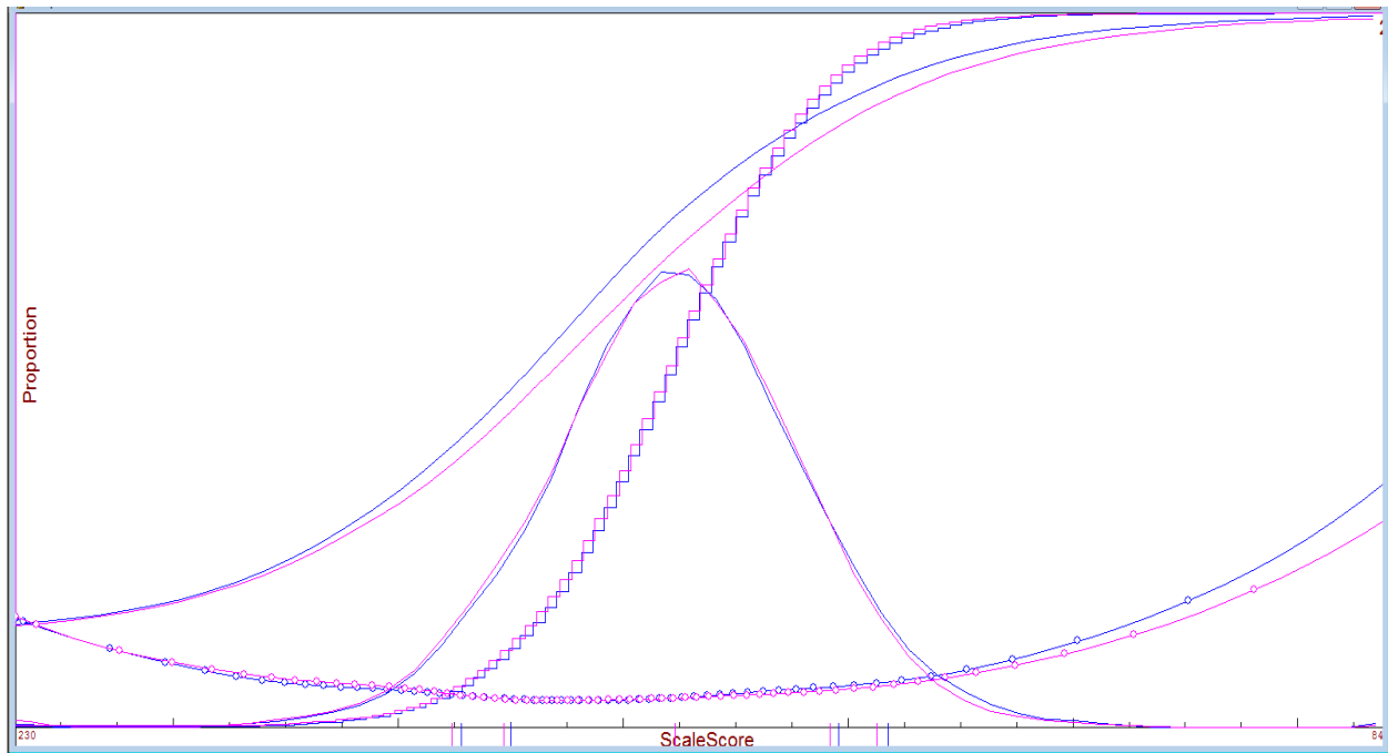
Figure 12. TCAP Grade 6 Writing Operational Tests
