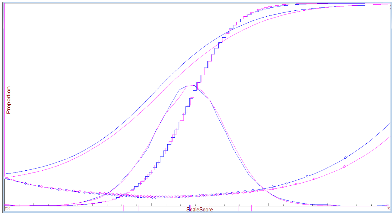
Figure 14. TCAP Grade 8 Writing Operational Tests
