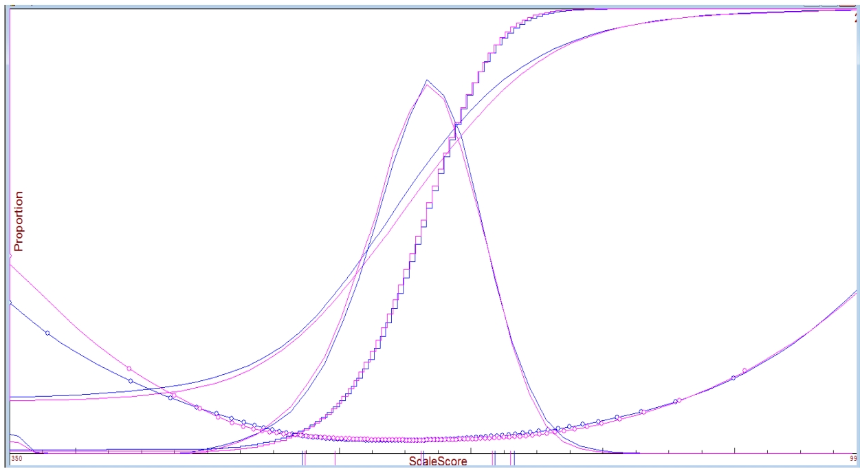
Figure 7. TCAP Grade 9 Reading Operational Tests
