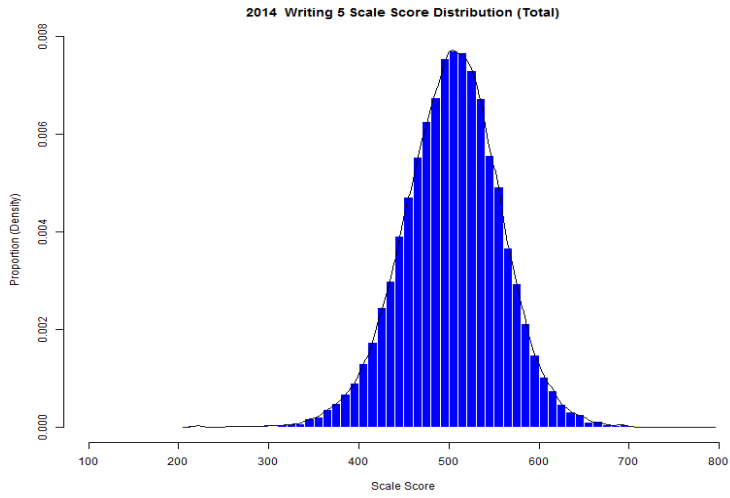
Figure 36. Grade 5 Writing Scale Score Distributions for the Total Population, Female, and Male Students
