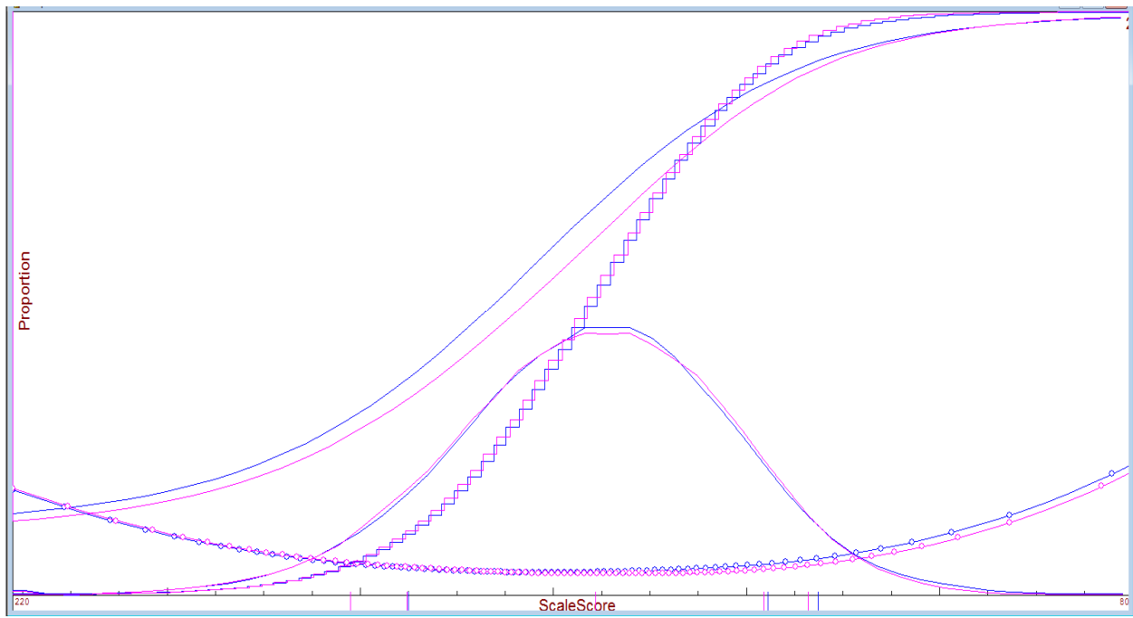
Figure 19. TCAP Grade 5 Mathematics Operational Tests
