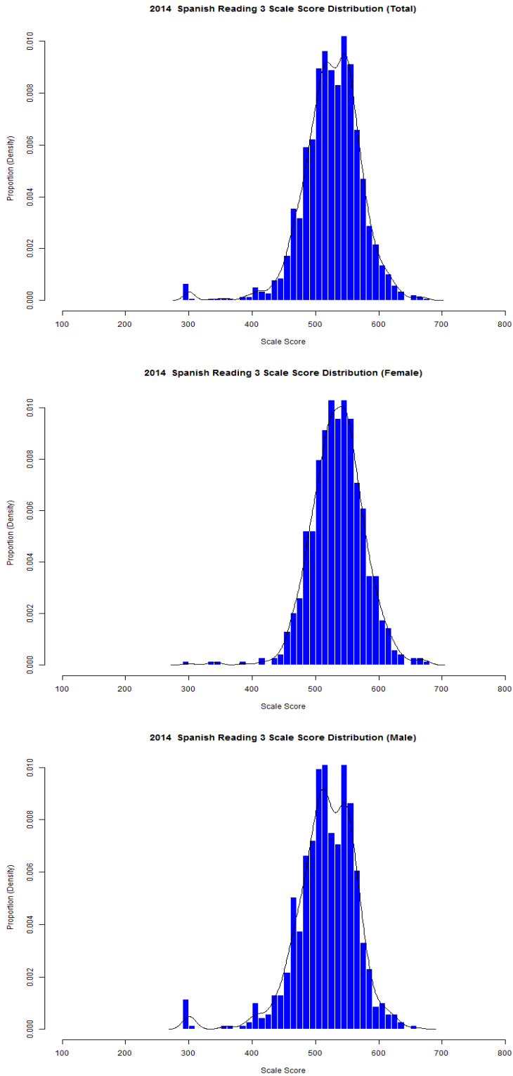
Figure 26. Grade 3 Reading (Spanish) Scale Score Distributions for the Total Population, Female, and Male Students
