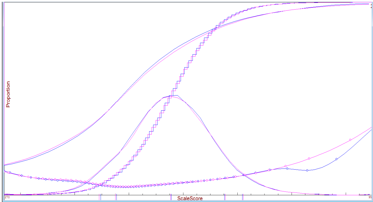
Figure 16. TCAP Grade 10 Writing Operational Tests
