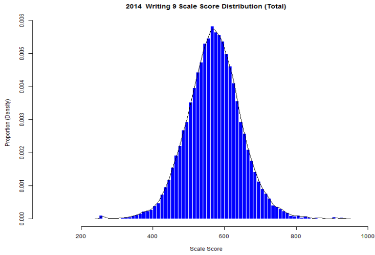
Figure 48. Grade 9 Writing Scale Score Distributions for the Total Population, Female, and Male Students
