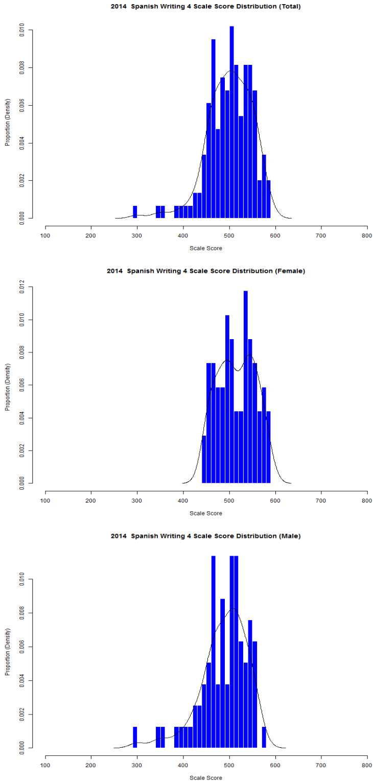
Figure 33. Grade 4 Writing (Spanish) Scale Score Distributions for the Total Population, Female, and Male Students
