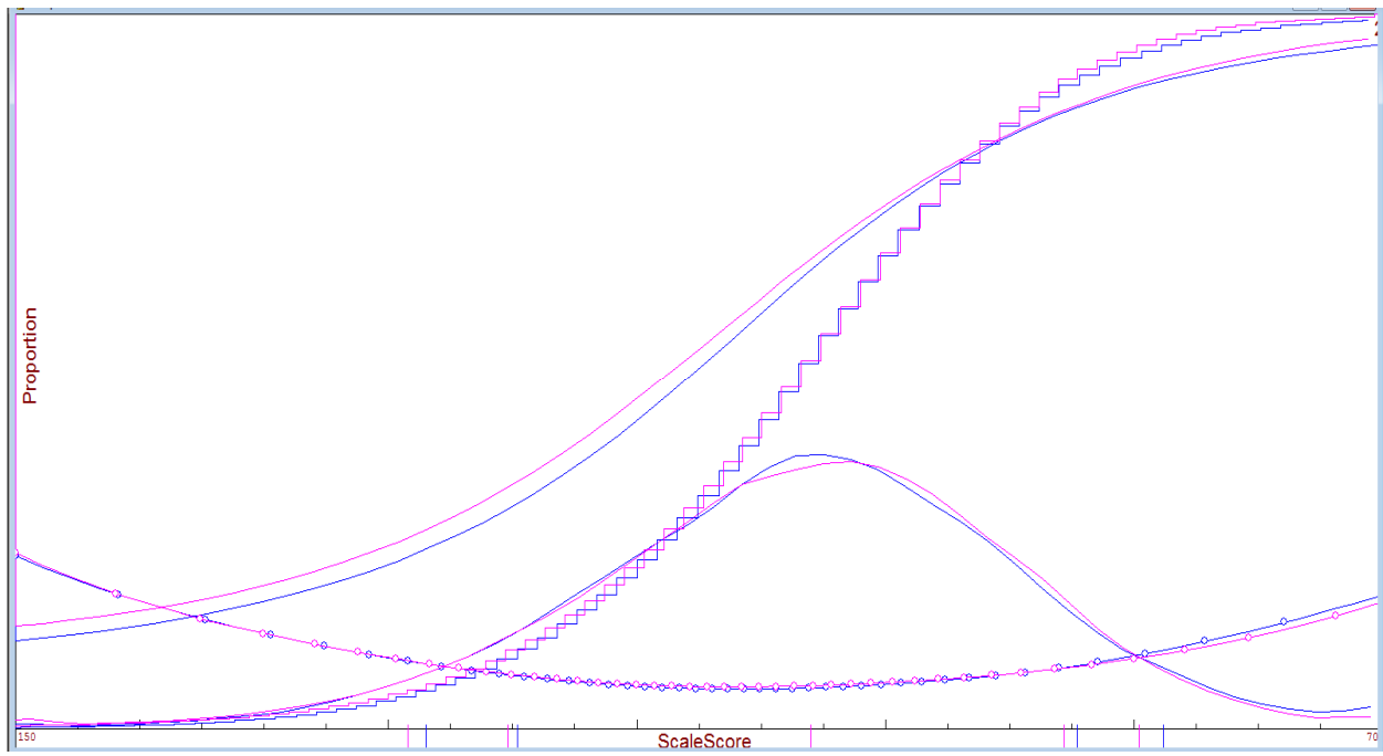
Figure 17. TCAP Grade 3 Mathematics Operational Tests
