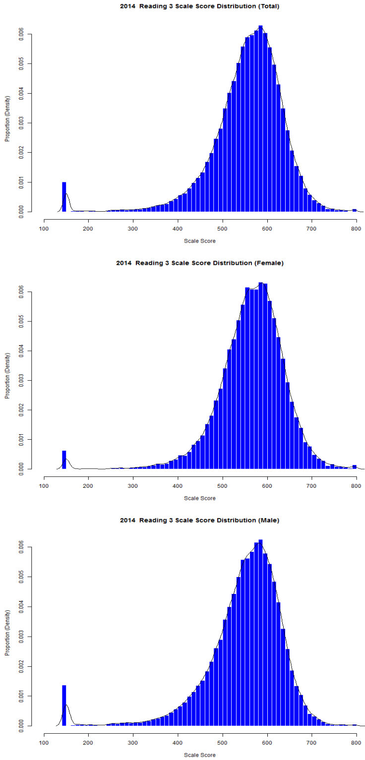
Figure 25. Grade 3 Reading Scale Score Distributions for the Total Population, Female, and Male Students
