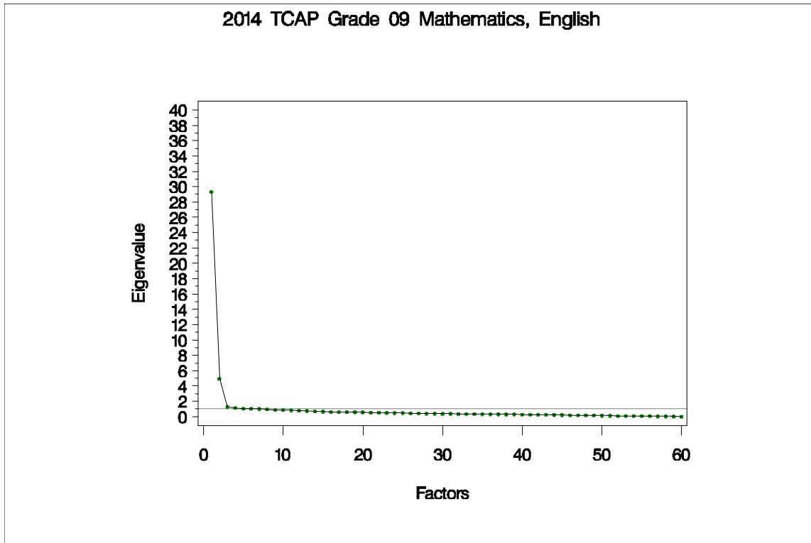
Figure 79. Eigenvalues and Proportions of Variance by Factor for TCAP Grade 9 Mathematics
