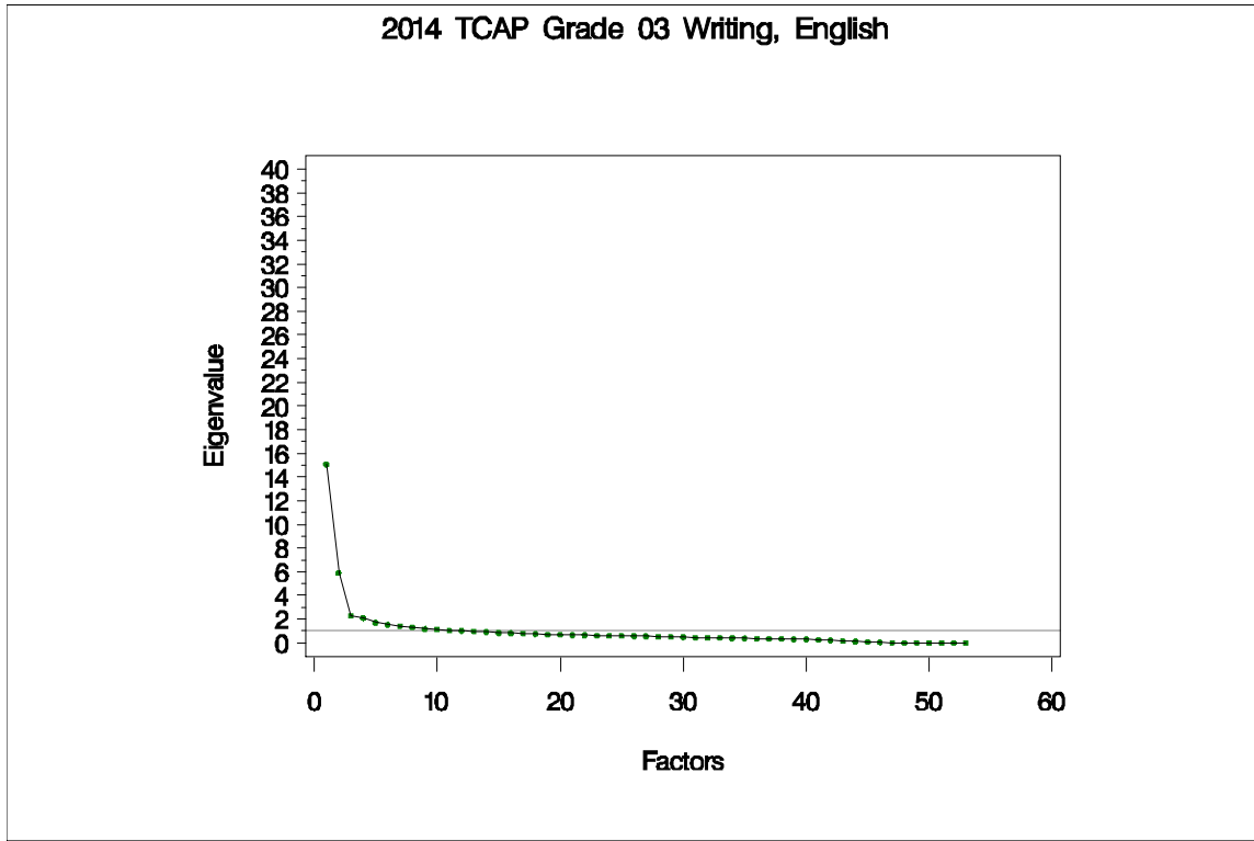
Figure 63. Eigenvalues and Proportions of Variance by Factor for TCAP Grade 3 Writing
