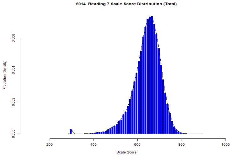
Figure 41. Grade 7 Reading Scale Score Distributions for the Total Population, Female, and Male Students
