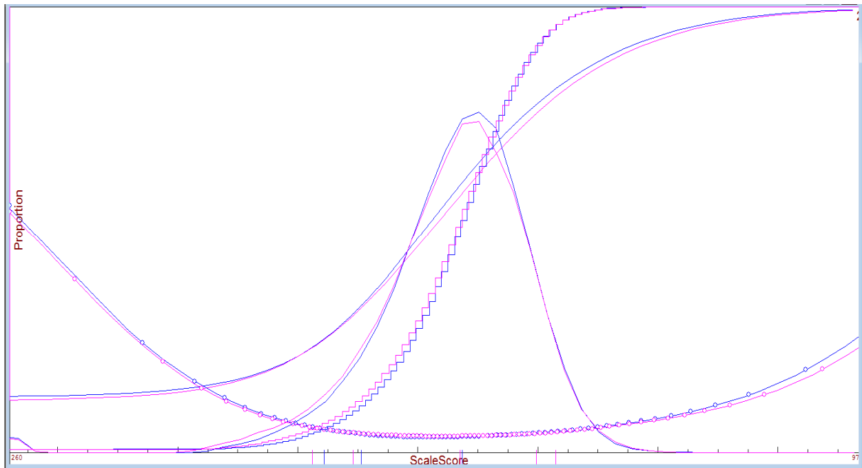
Figure 4. TCAP Grade 6 Reading Operational Tests
