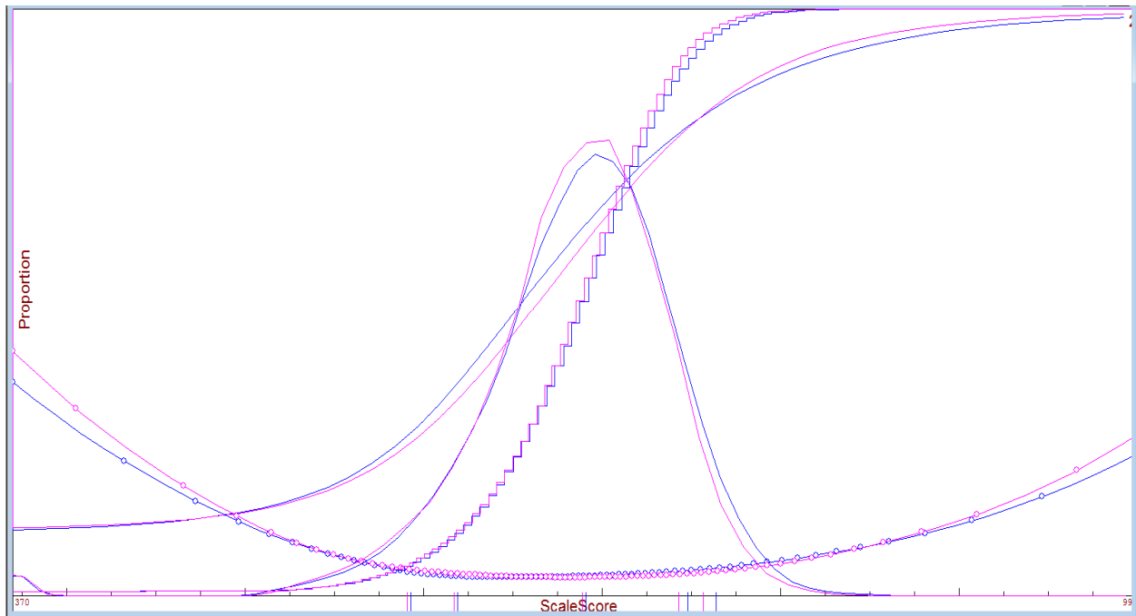
Figure 8. TCAP Grade 10 Reading Operational Tests
