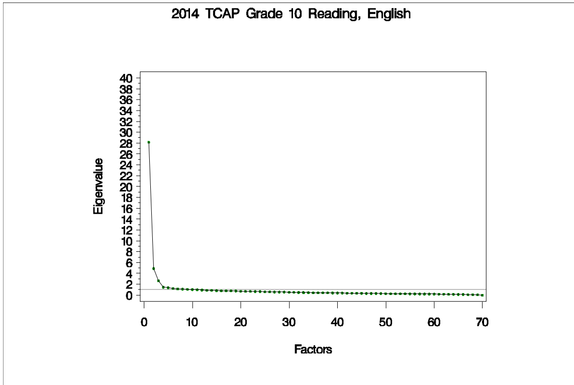
Figure 62. Eigenvalues and Proportions of Variance by Factor for TCAP Grade 10 Reading
