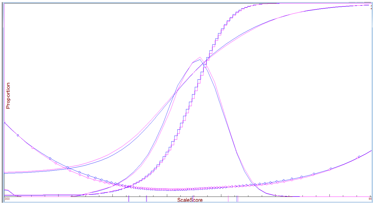
Figure 5. TCAP Grade 7 Reading Operational Tests
