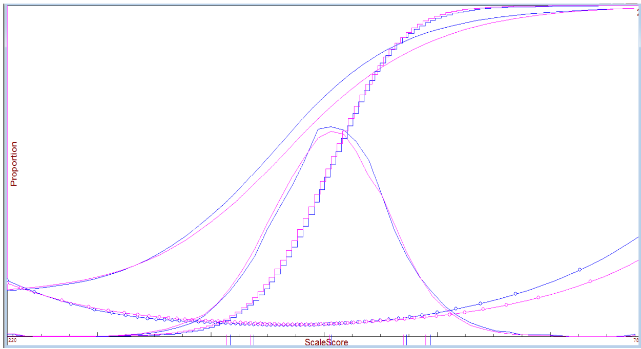
Figure 11. TCAP Grade 5 Writing Operational Tests
