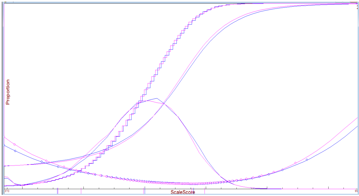
Figure 24. TCAP Grade 10 Mathematics Operational Tests
