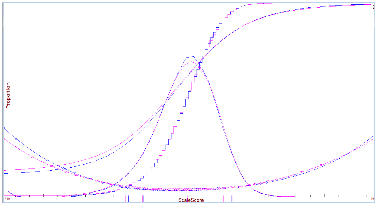
Figure 6. TCAP Grade 8 Reading Operational Tests
