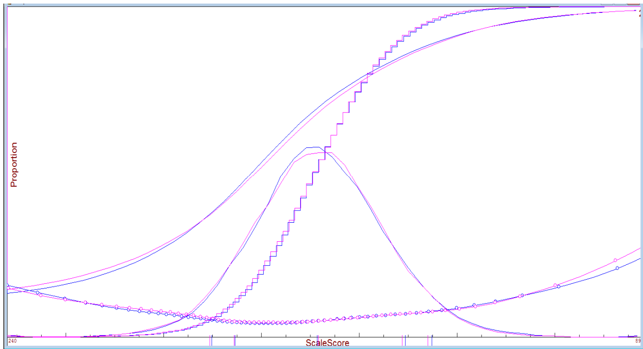
Figure 13. TCAP Grade 7 Writing Operational Tests
