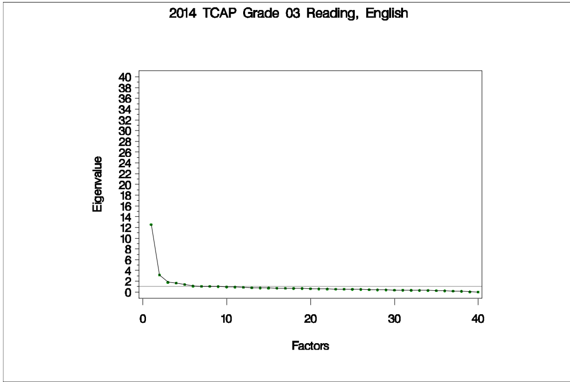
Figure 53. Eigenvalues and Proportions of Variance by Factor for TCAP Grade 3 Reading
