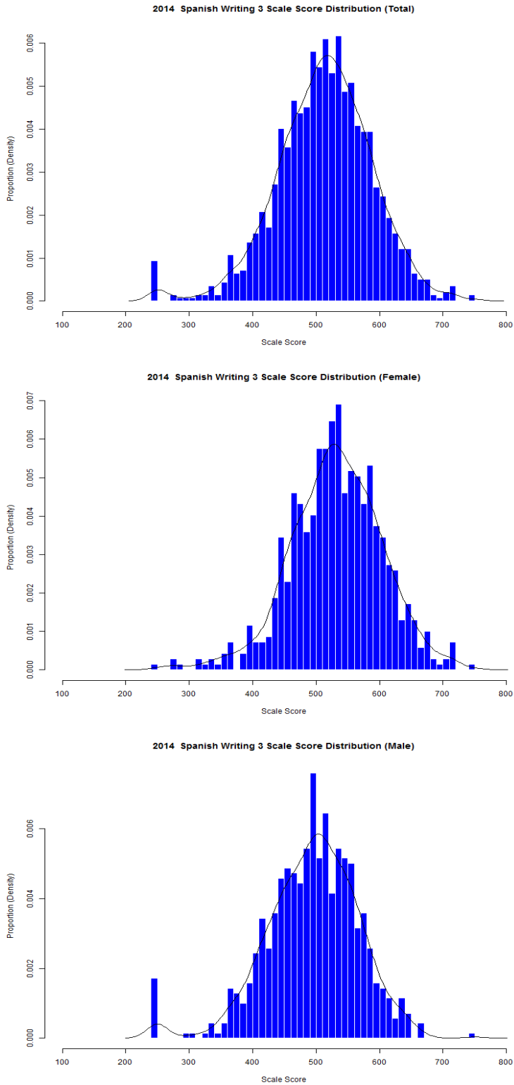
Figure 28. Grade 3 Writing (Spanish) Scale Score Distributions for the Total Population, Female, and Male Students
