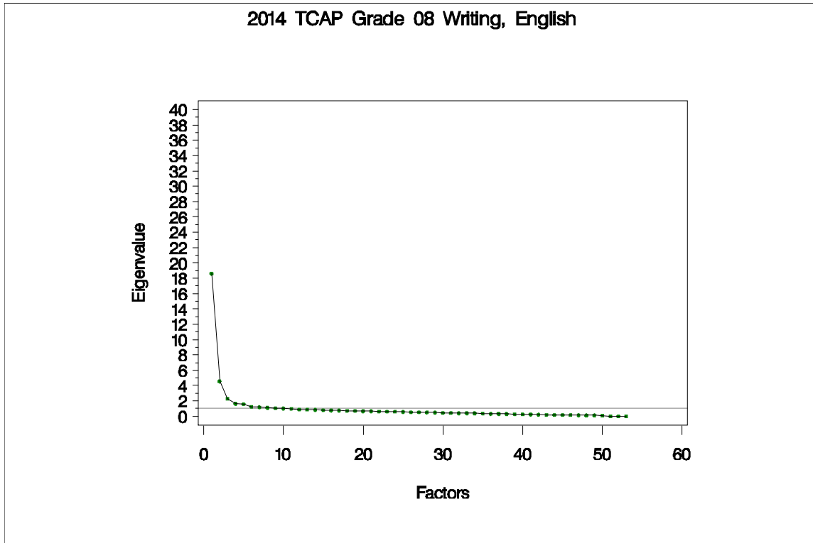
Figure 70. Eigenvalues and Proportions of Variance by Factor for TCAP Grade 8 Writing
