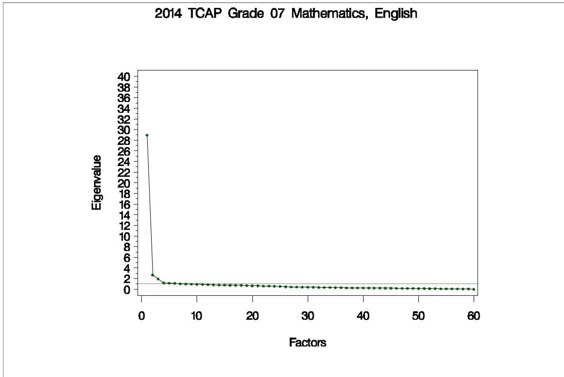
Figure 77. Eigenvalues and Proportions of Variance by Factor for TCAP Grade 7 Mathematics
