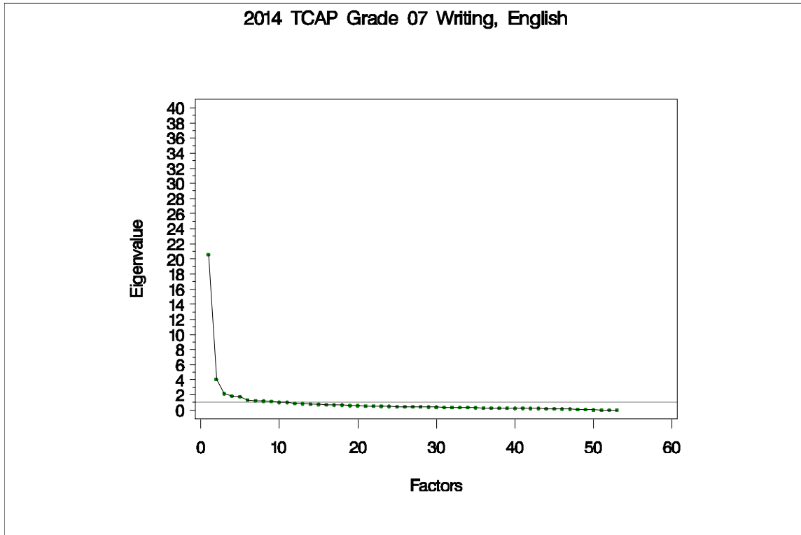
Figure 69. Eigenvalues and Proportions of Variance by Factor for TCAP Grade 7 Writing
