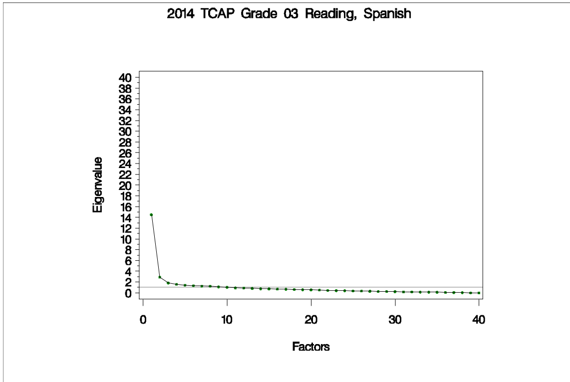
Figure 54. Eigenvalues and Proportions of Variance by Factor for TCAP Grade 3 Reading (Spanish)
