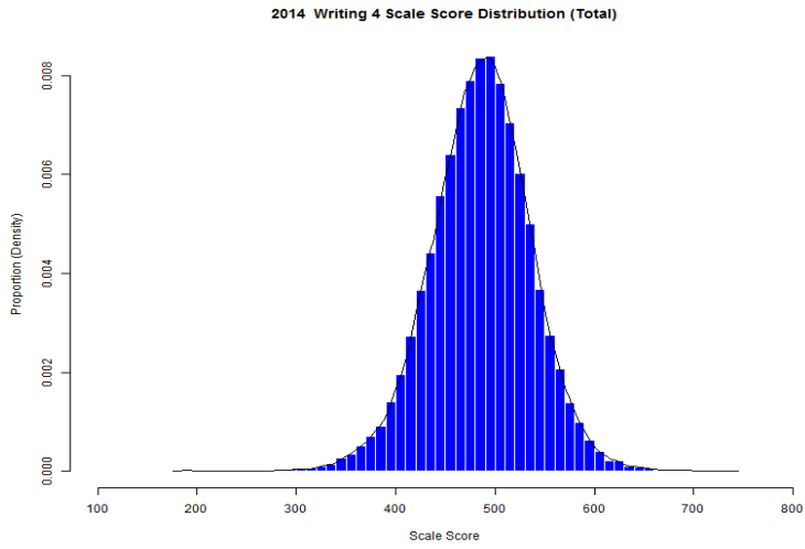
Figure 32. Grade 4 Writing Scale Score Distributions for the Total Population, Female, and Male Students
