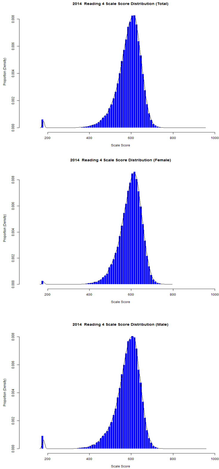
Figure 30. Grade 4 Reading Scale Score Distributions for the Total Population, Female, and Male Students
