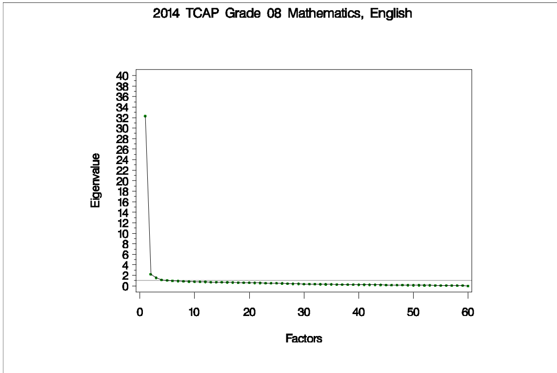
Figure 78. Eigenvalues and Proportions of Variance by Factor for TCAP Grade 8 Mathematics
