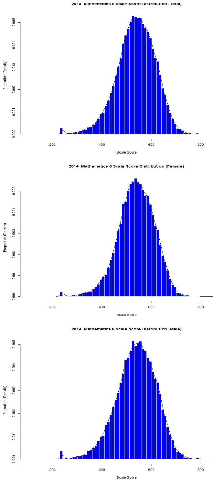
Figure 40. Grade 6 Mathematics Scale Score Distributions for the Total Population, Female, and Male Students
