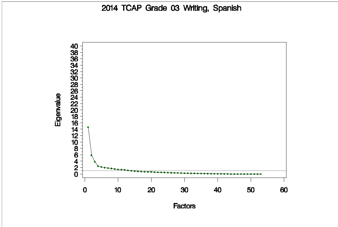
Figure 64. Eigenvalues and Proportions of Variance by Factor for TCAP Grade 3 Writing (Spanish)
