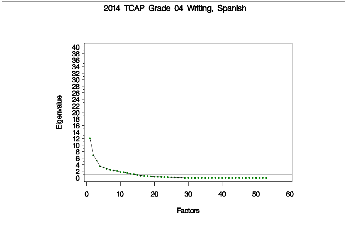
Figure 66. Eigenvalues and Proportions of Variance by Factor for TCAP Grade 4 Writing (Spanish)
