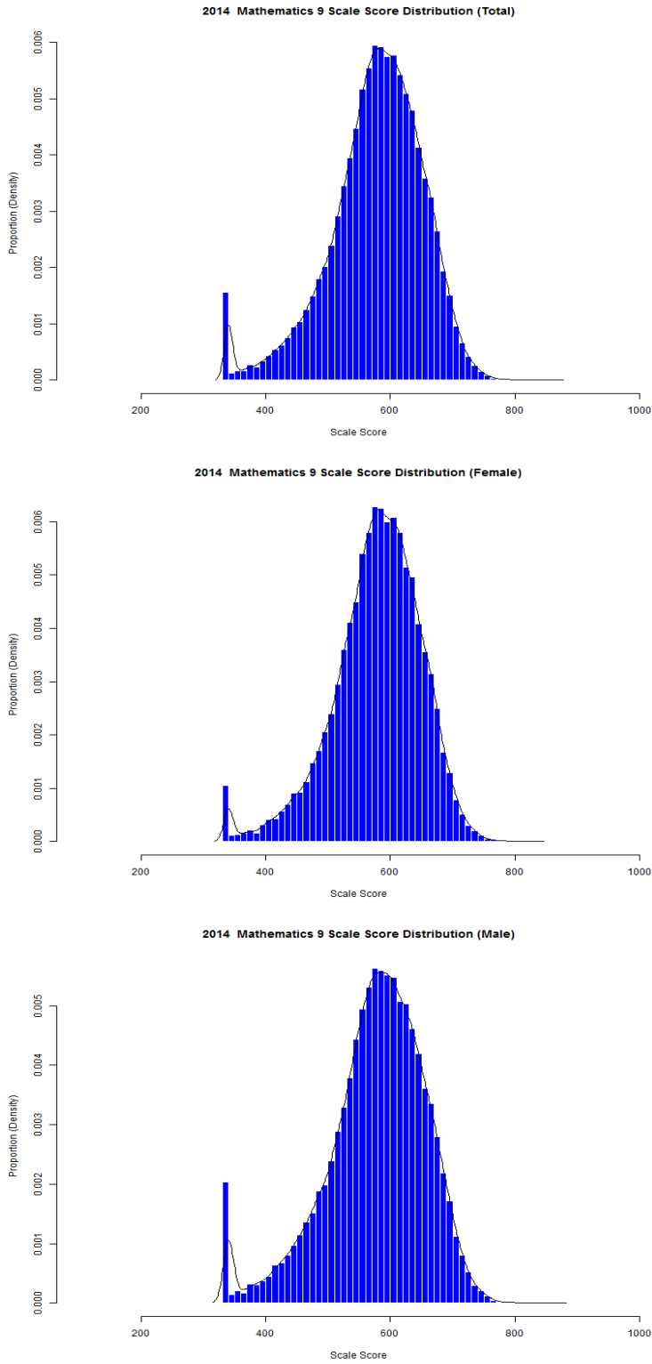
Figure 49. Grade 9 Mathematics Scale Score Distributions for the Total Population, Female, and Male Students
