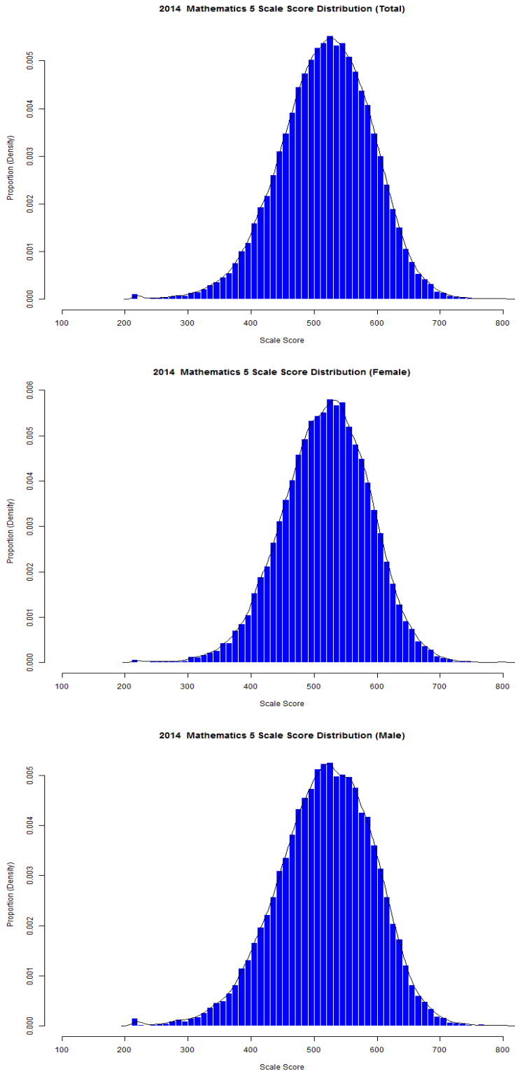
Figure 37. Grade 5 Mathematics Scale Score Distributions for the Total Population, Female, and Male Students
