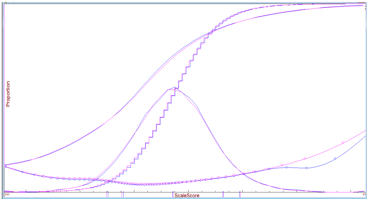
Figure 15. TCAP Grade 9 Writing Operational Tests
