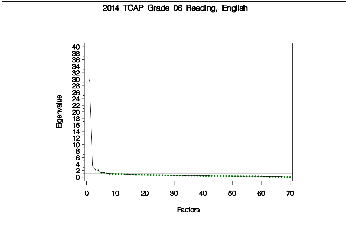
Figure 58. Eigenvalues and Proportions of Variance by Factor for TCAP Grade 6 Reading
