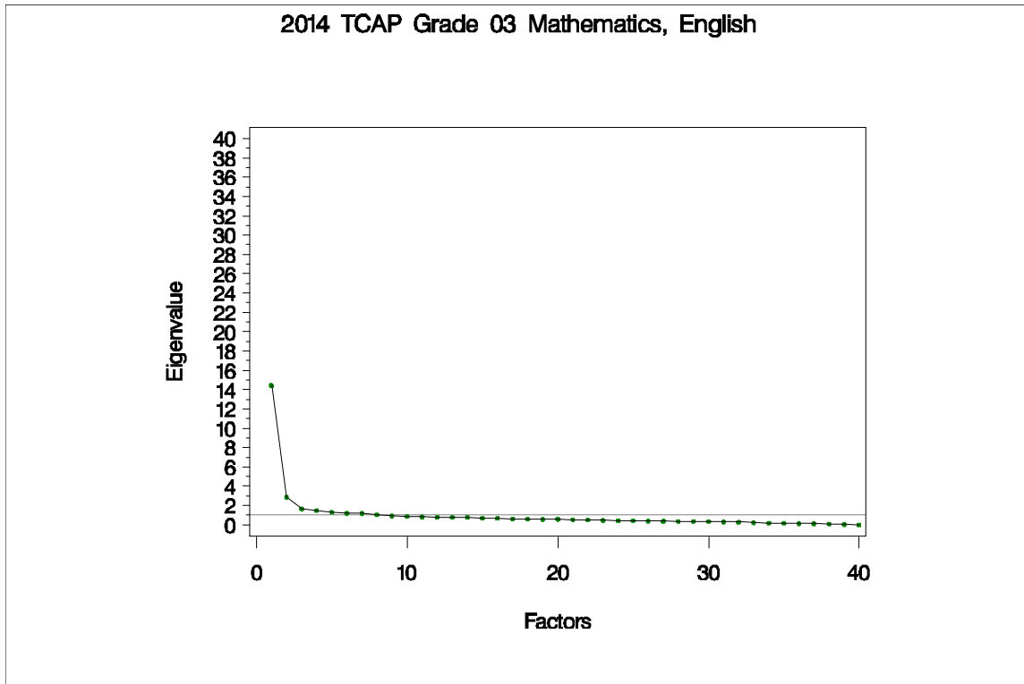
Figure 73. Eigenvalues and Proportions of Variance by Factor for TCAP Grade 3 Mathematics
