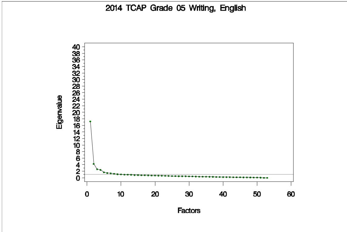
Figure 67. Eigenvalues and Proportions of Variance by Factor for TCAP Grade 5 Writing
