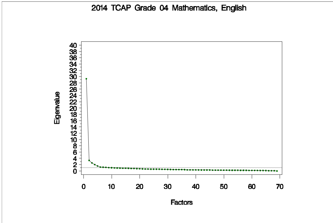
Figure 74. Eigenvalues and Proportions of Variance by Factor for TCAP Grade 4 Mathematics
