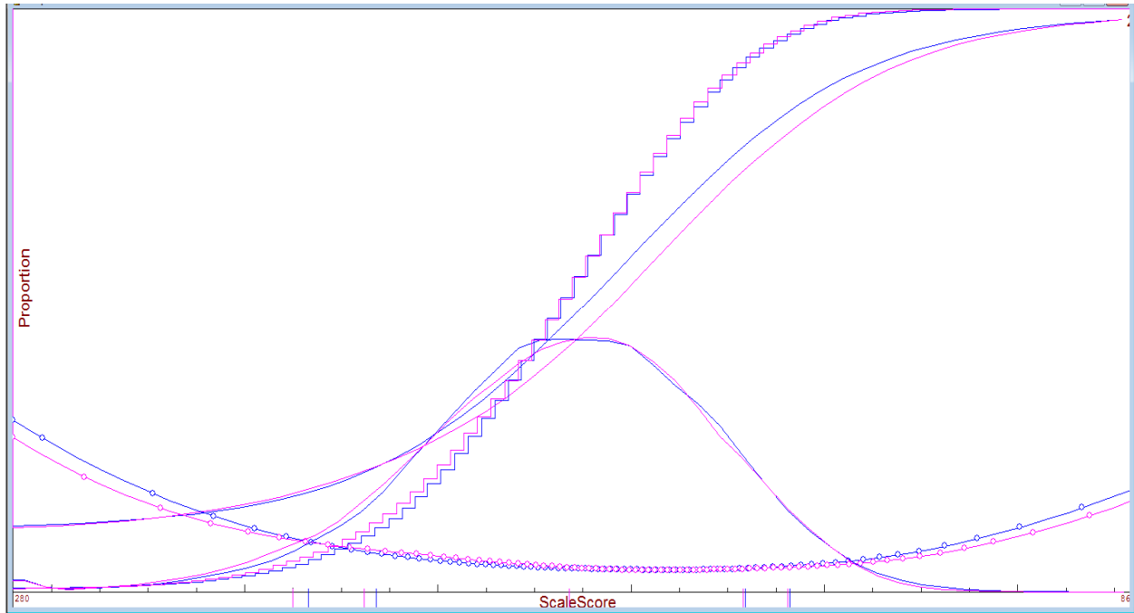
Figure 21. TCAP Grade 7 Mathematics Operational Tests
