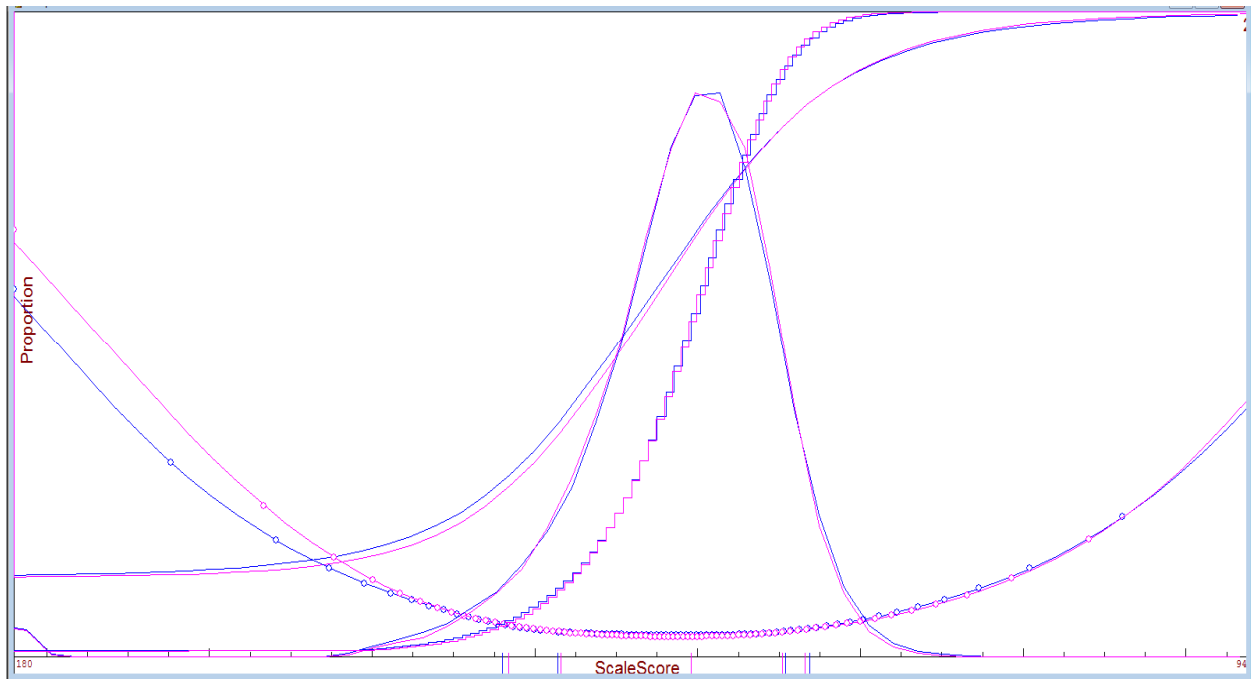
Figure 2. TCAP Grade 4 Reading Operational Tests
