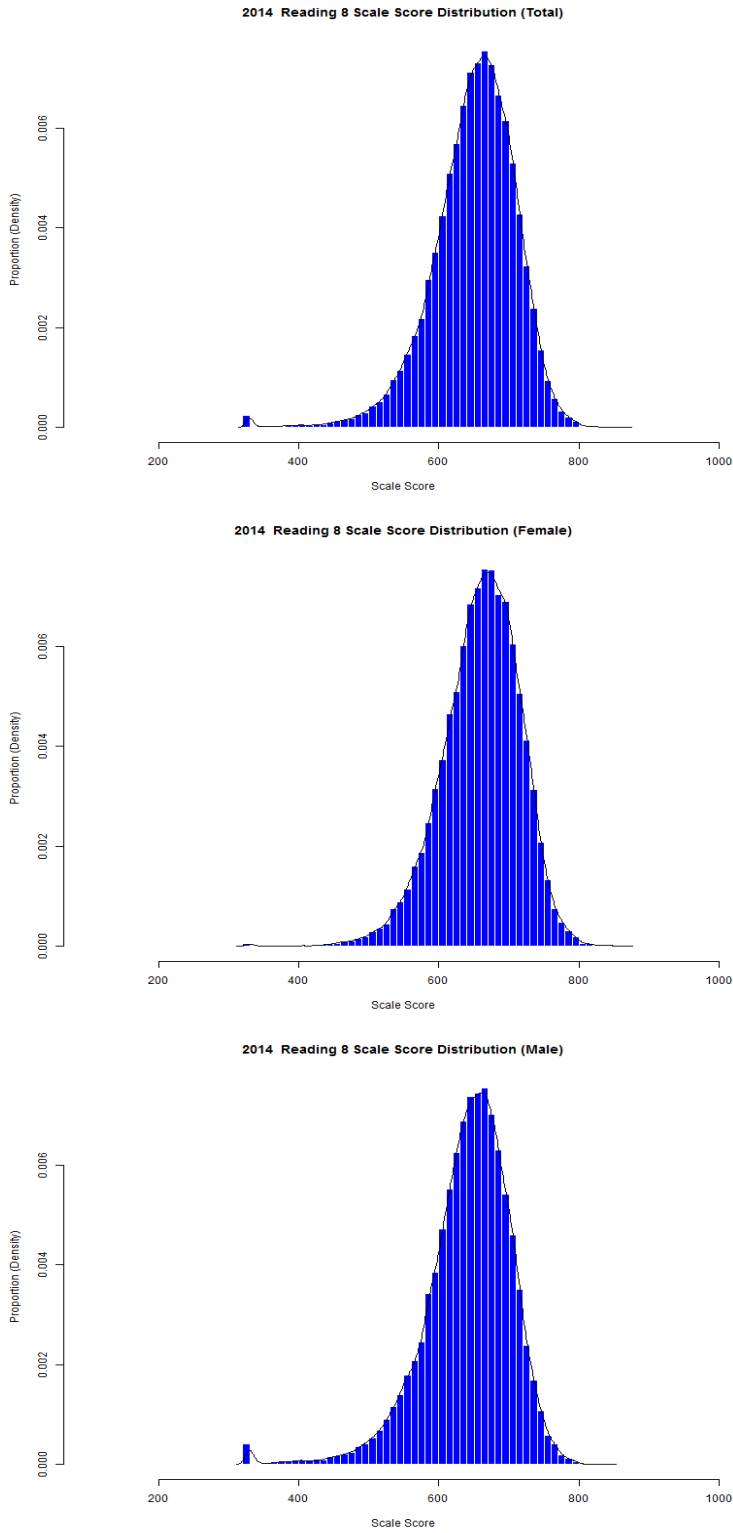
Figure 44. Grade 8 Reading Scale Score Distributions for the Total Population, Female, and Male Students
