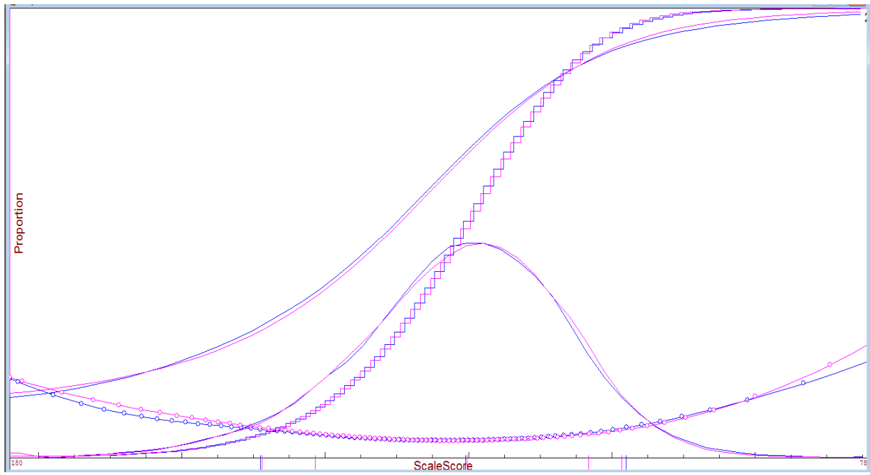
Figure 18. TCAP Grade 4 Mathematics Operational Tests
