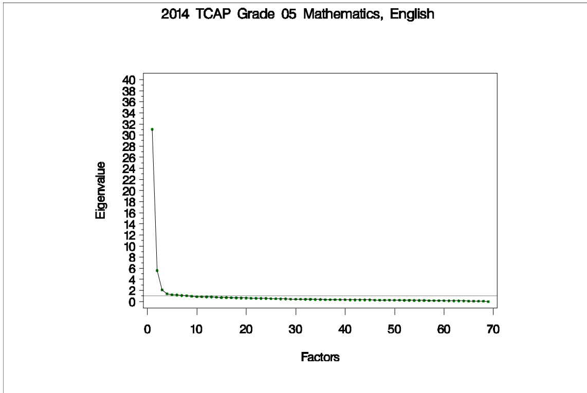
Figure 75. Eigenvalues and Proportions of Variance by Factor for TCAP Grade 5 Mathematics
