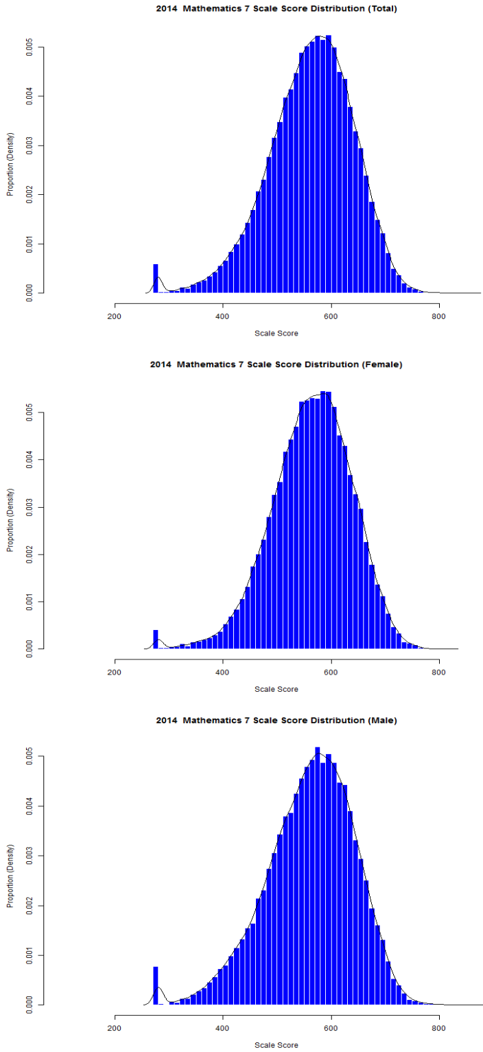
Figure 43. Grade 7 Mathematics Scale Score Distributions for the Total Population, Female, and Male Students
