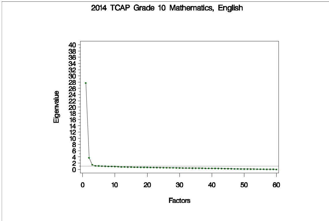
Figure 80. Eigenvalues and Proportions of Variance by Factor for TCAP Grade 10 Mathematics
