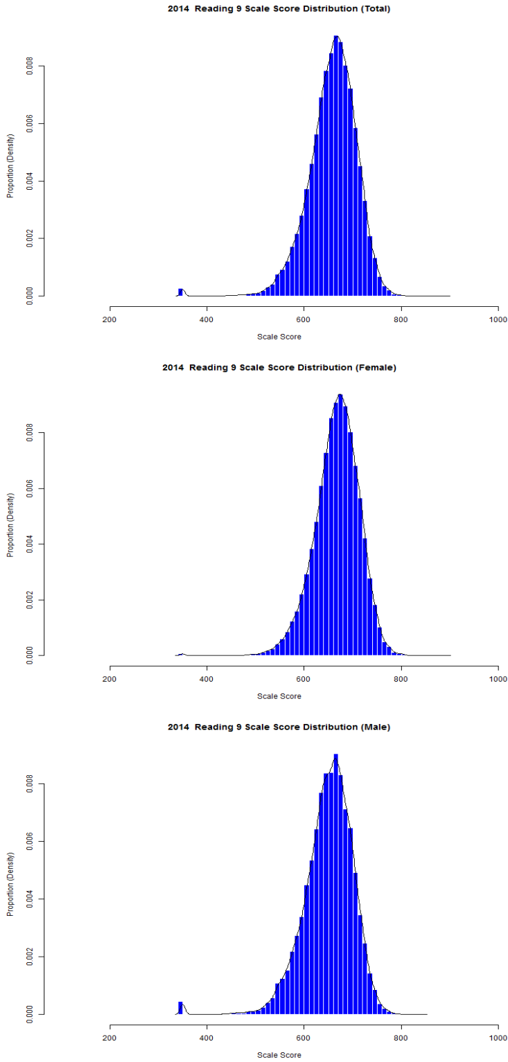
Figure 47. Grade 9 Reading Scale Score Distributions for the Total Population, Female, and Male Students
