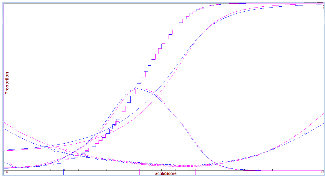
Figure 23. TCAP Grade 9 Mathematics Operational Tests
